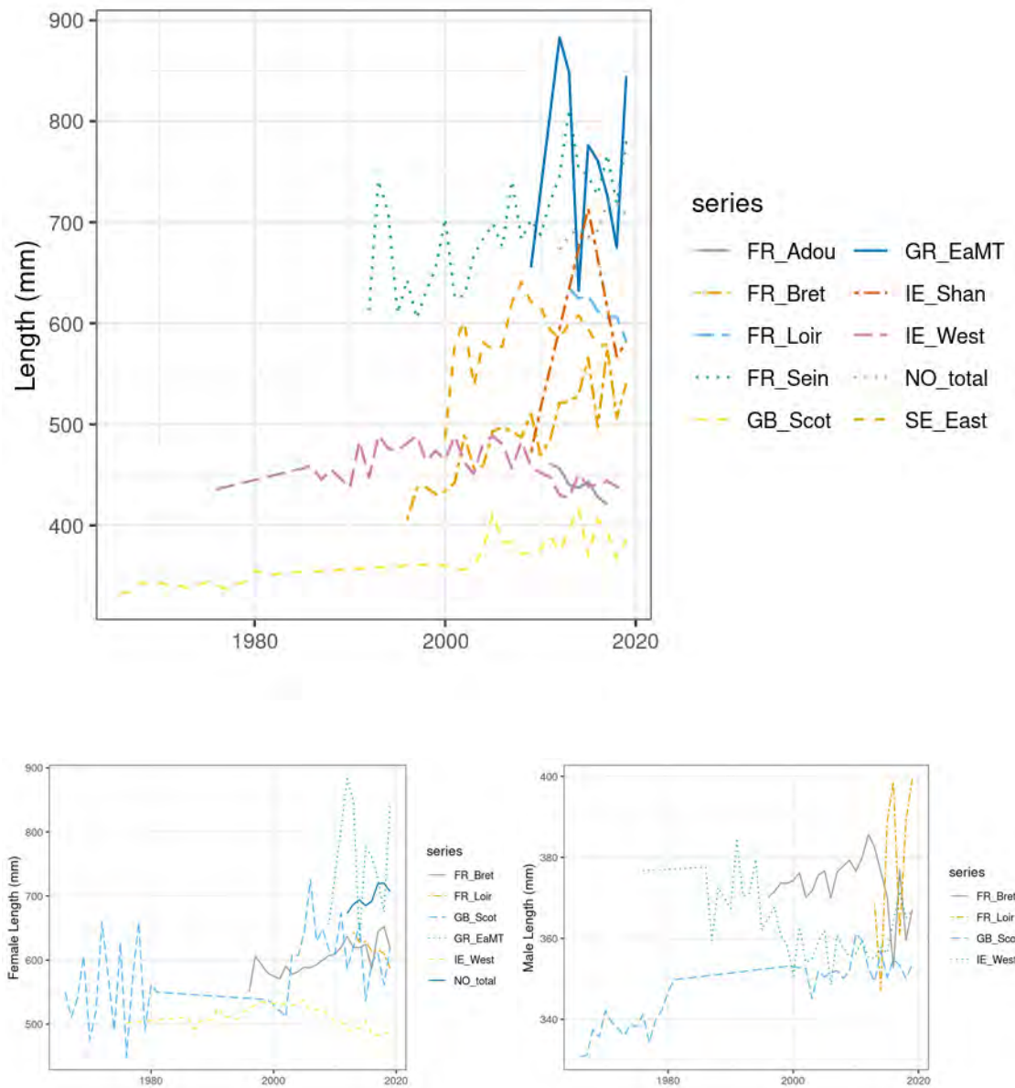
Figure 14. Silver series temporal trends in annual average annual length (above both sexes included, below per sex).
