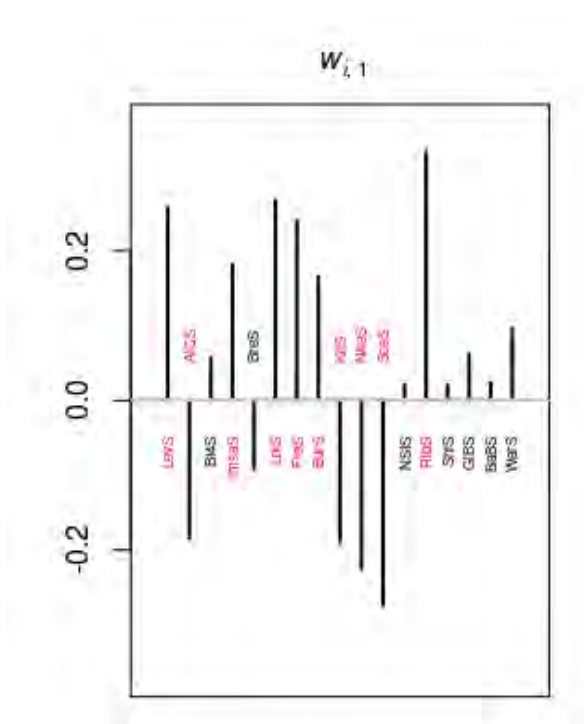
Figure 3.2.17. Factor loadings of the silver eel DFA (red names stand for loadings absolute values greater than 0.1).
