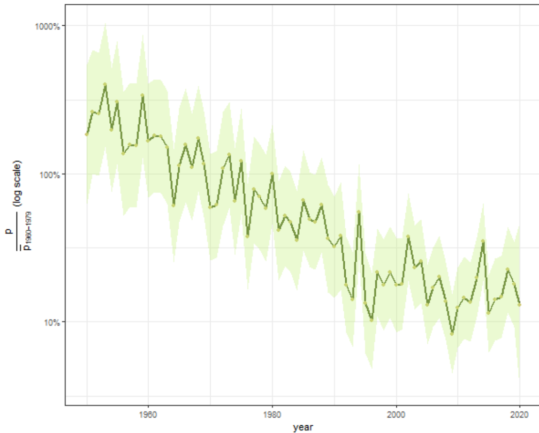
Figure 3.1.6. Yellow eel GLM recruitment trend and 95% confidence interval for Europe updated to 2020. The GLM ( yellow eel ~ year + site ) was fitted to 16 yellow eel time-series ( p ) and scaled to the 1960–1979 average \bar{p}_{1960-1979} (the dashed line). Note the log scale.
