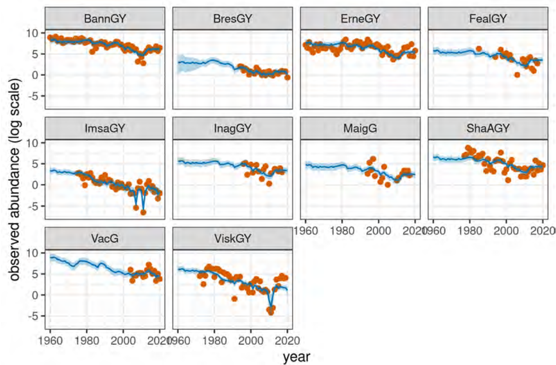
Figure 7. Model fits to trap time-series. Blue lines indicate medians of the posterior distributions of the value predicted by the model, and blue ribbons corresponding 95% credibility interval. Red dots stands for observations. Each panel corresponds to one of the time-series used in the model.
