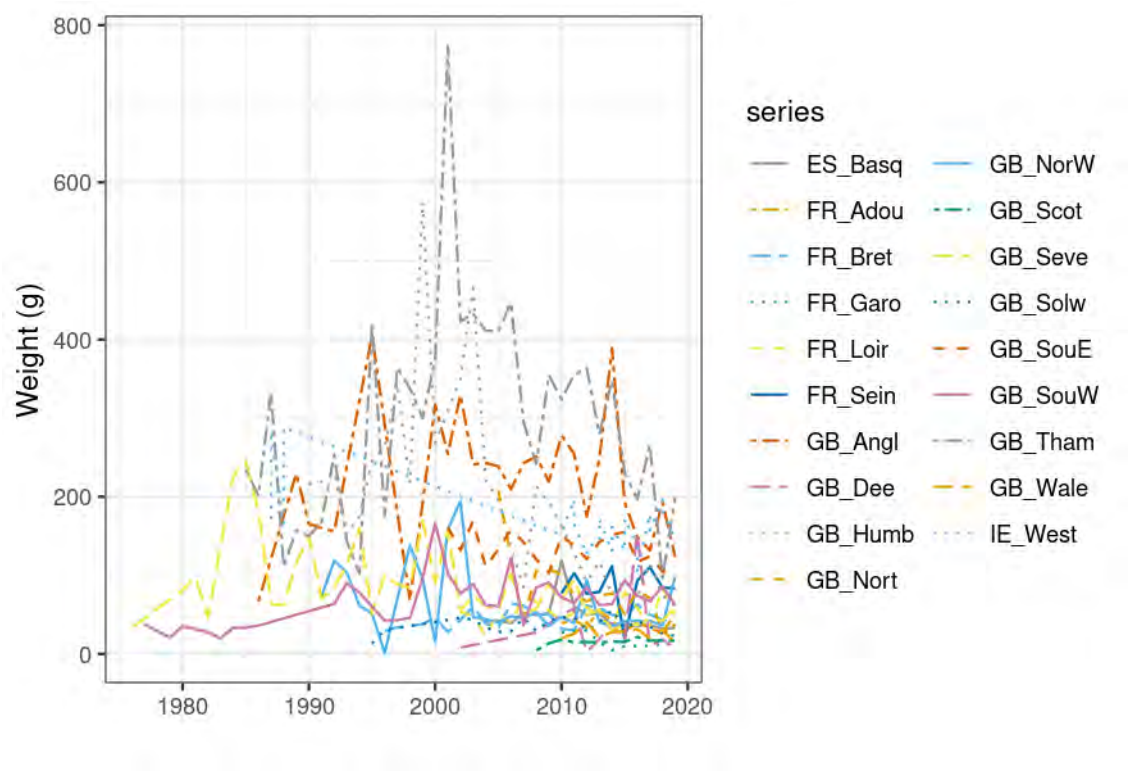
Figure 13. Yellow series temporal trends in average annual weight.
