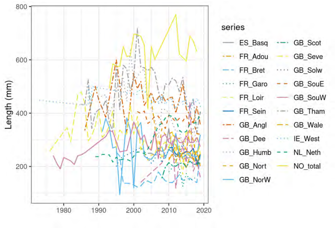
Figure 12. Yellow series temporal trends in average annual length.
