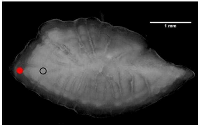
Figure 4.23. Otolith of a T. mediterraneus specimen (age: 0, TL: 12.5 cm, caught in early spring). The open black circle is a false ring; the red circle is the first winter ring (Carbonara and Follesa, 2018).
