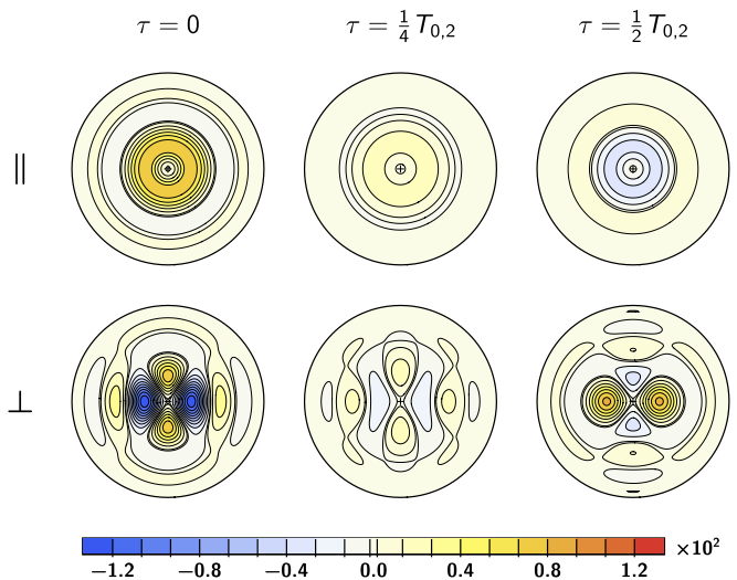
FIG. 5. Series of difference scattering patterns (pump on – pump off) that correspond to the detector images shown in Fig. 4. The static scattering signal for the rotational eigenstate with quantum numbers (J, M) = (0, 0) (see Fig. 2, left column) is subtracted.
