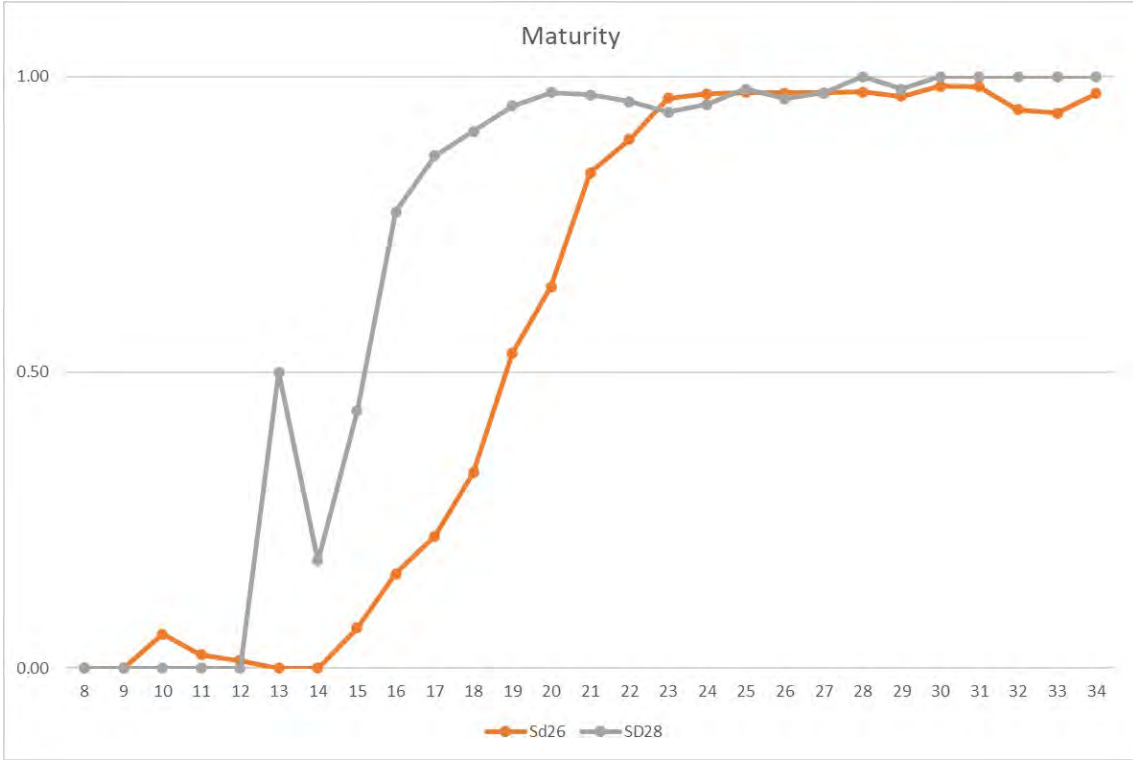
Figure 3.4.10. Flounder in subdivisions 26 and 28 (Eastern Gotland and Gulf of Gdansk). Proportion of mature flounder females by Subdivisions, BIT Survey in 4th Quarters from 2014-2019.
