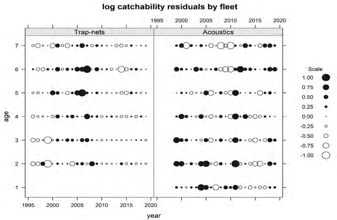
Figure 4.3.8b. Gulf of Riga herring. Log catchability residuals of trap-net fleet (left) and hydro-acoustics fleet (right).
