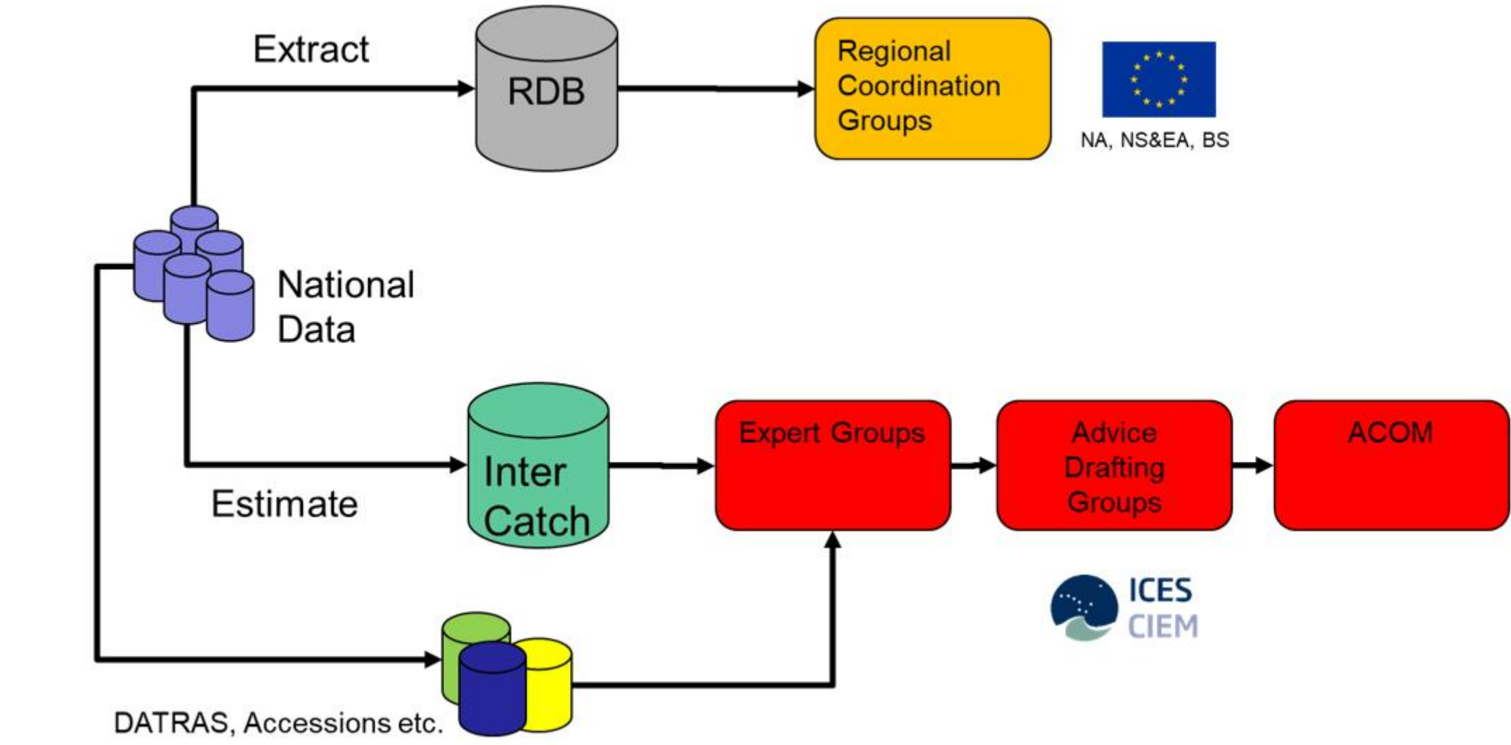
Current data pipeline incorporating the existing Regional Database (RDB) and ICES InterCatch systems
