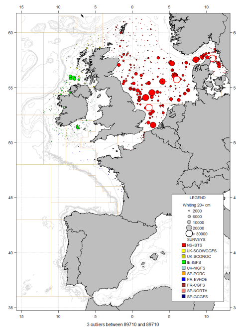
Figure A.6.25. Catches in numbers per hour of 1+ group whiting, Merlangius merlangus (≥20 cm), in summer/autumn 2020 IBTSurveys.
