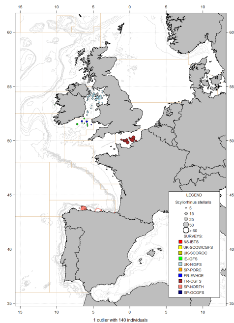
Figure A.6.30. Catches in numbers per hour of nurse hound, Scyliorhinus stellaris , in summer/autumn 2020 IBTSurveys.
