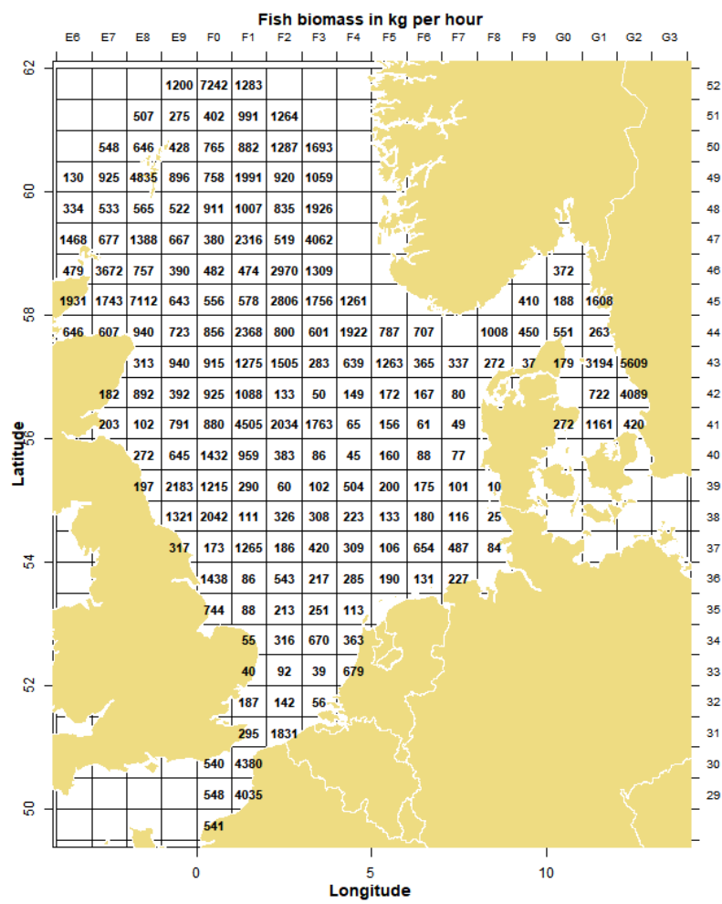
Figure A3.2 - Distribution of fish biomass in IBTS hauls by rectangle in the North Sea, Q1 2021 (values standardized to kg per hour haul duration; mean per rectangle).
