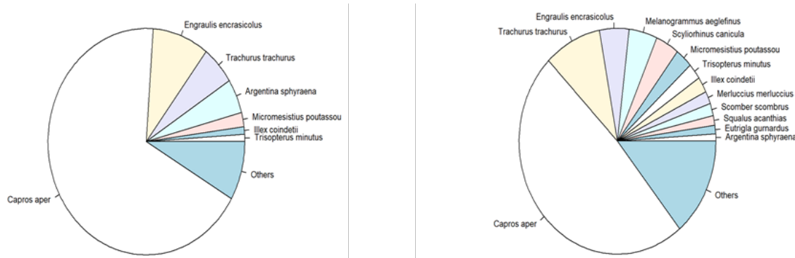
Figure A.5.12.2 - Species dominance over the entire "EVHOE" sampled area in term of A) abundance and B) biomass.
