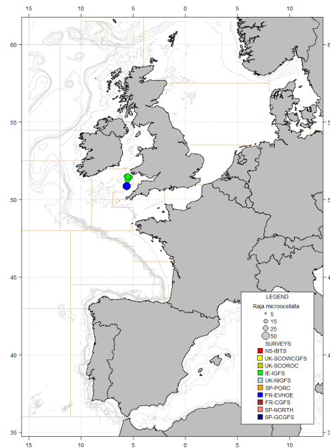
Figure A.6.37. Catches in numbers per hour per hour of small eyed ray, Raja microcellata , in summer/autumn 2018 IBTSurveys.
