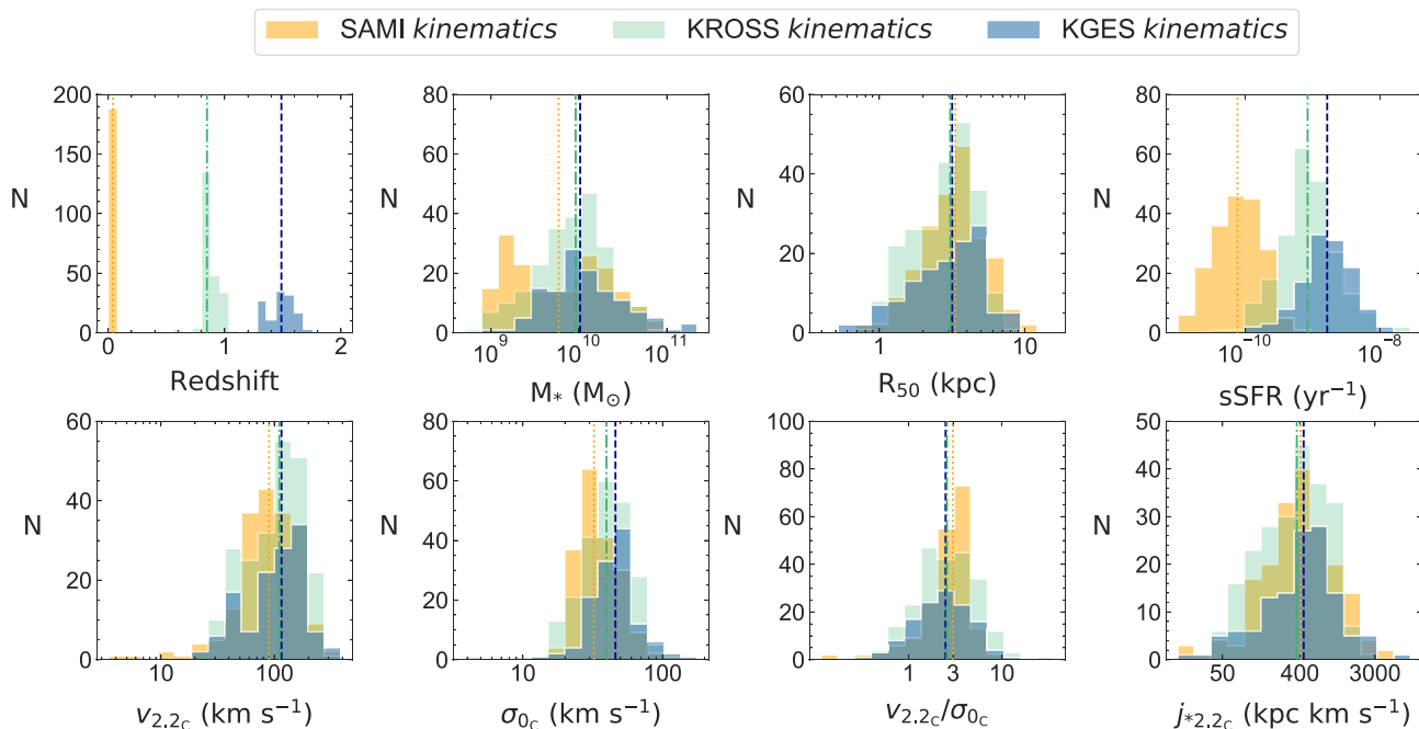
Figure 5. The distributions of key properties of star-forming galaxies in our kinematics sub-samples at z \approx 1.5 (KGES), z \approx 0.9 (KROSS), and z \approx 0.04 (SAMI). The median of each distribution is shown as a dashed vertical line in the corresponding colour. The key properties of normal (massive) star-forming galaxies are surprisingly constant with redshift, aside from significantly elevated sSFRs and gas velocity dispersions with increasing redshift (as judged by formal comparison of the median values between redshifts, in each case).
