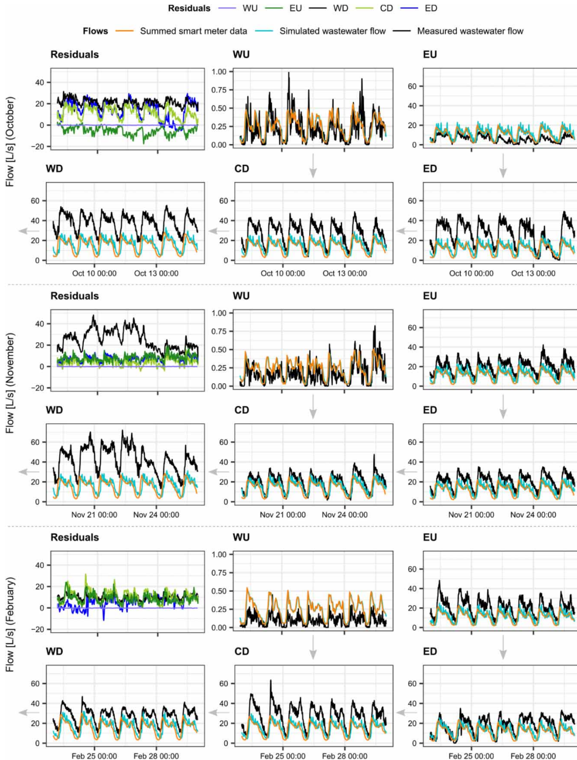
Figure 6 | Summed smart meter data ( Q_{SM} ) and simulated ( Q_{sim} ) and observed ( Q_{obs} ) sewage flows in October (top panel, Mon-Sat), November (middle panel, Mon-Sun) and February (lower panel, Sat-Fri) (Equation (1)). All data are in local time. For Q_{sim} and Q_{obs} , a 30 min moving average filter has been applied for better readability. Notice the different scales used for Residuals, WU and the four remaining plots. Due to the small flow in WU, the residuals appear constant in the Residuals plot.
