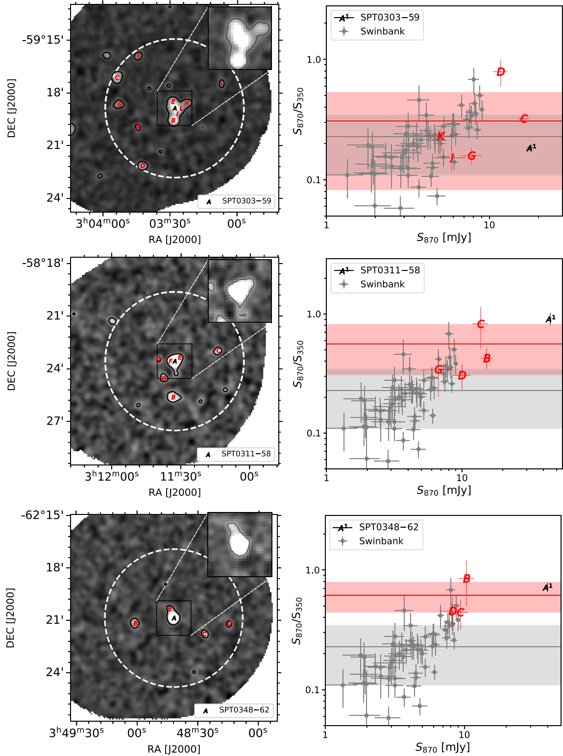
Figure 5. Spatial distributions and colours of sources in each field. Left: The grey-scale image shows the 18.6-arcsec-convolved 870-μm LABOCA map. The objects overlaid on these images are the sources within our 240 arcsec cutoff labelled accordingly to Appendix A. Contours corresponding to 3.7\sigma are displayed in black, while the white dotted-circle represents the radial cutoff. Insets show enlarged areas of the central core (12 arcsec on a side) convolved LABOCA map. Right: Flux density ratio versus flux density plot. The sources are labelled the same as on the LABOCA maps, but we show the integrated colour-brightness point for the extended central core with integer superscripts. We compare the average colours of our fields to the sample of SMGs from Swinbank et al. (2014) (light grey) and show that our sources have higher colours.
