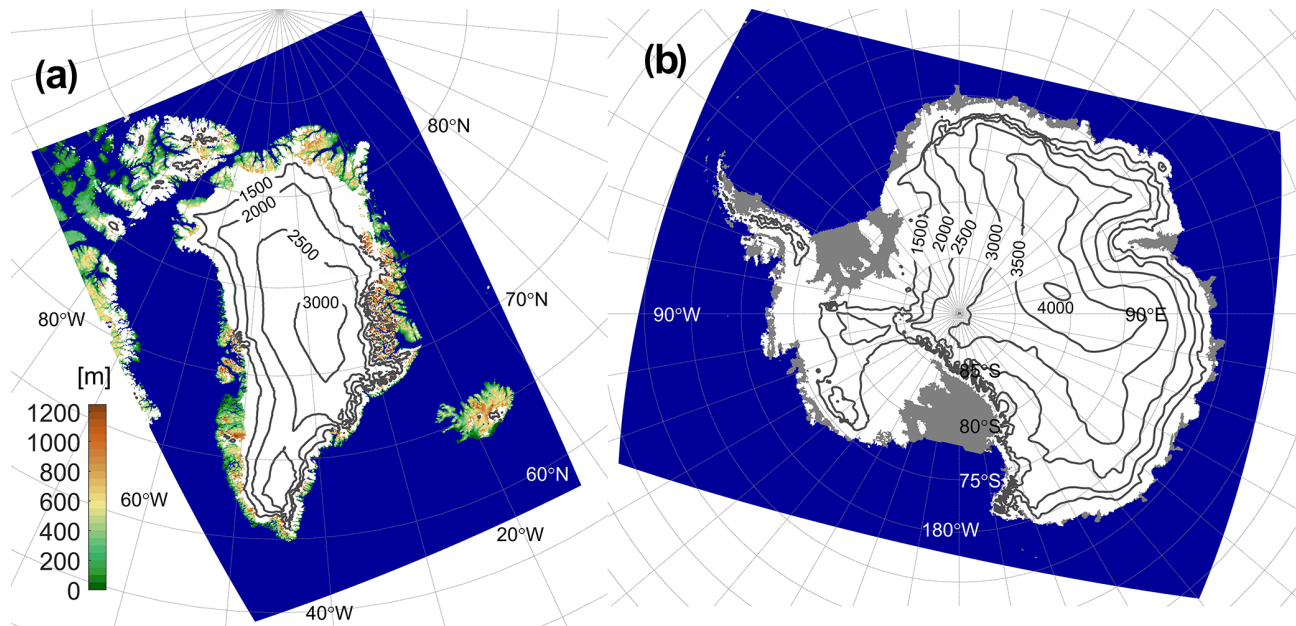
Figure 1. Topography for the two model domains. Sea points are given in blue; non-glacial land grid points are given in green and brown; Antarctic ice shelves are given in grey, while glacial points are given in white with surface elevation contour lines added. The Greenland domain (a) has a model resolution of about 5.5 km (0.05°), while the Antarctica domain (b) has a model resolution of about 12.5 km (0.11°).
