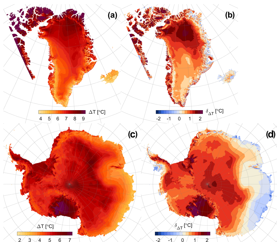
Figure 5. Change in 2 m temperature for Greenland for 2081–2100 relative to 1991–2010 for the EC-Earth v3 SSP5-8.5 scenario (a). Difference in the change in 2 m temperature for EC-Earth3 SSP5-8.5 relative to EC-Earth2 RCP8.5 (b). Change in 2 m temperature for Antarctica for 2071–2100 relative to 1971–2000 for the SSP5-8.5 scenario (c). Difference in the change in 2 m temperature for SSP5-8.5 relative to RCP8.5 (d). Note that the colour bar limits in panels (a) and (c) differ.
