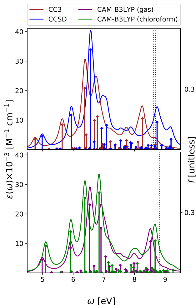
Fig. 4 Cytosine. Upper panel : OPA at EOM-CCSD/aug-cc-pVDZ and EOM-CC3/aug-cc-pVDZ levels in gas phase. Bottom panel : OPA at CAM-B3LYP/aug-cc-pVDZ level of theory in gas phase and in chloroform solution. Geometry optimized in the gas phase enforcing C_s symmetry. The vertical lines indicate the first ionisation energy in the gas phase ( \Delta SCF at DFT level). HWHM = 0.0045563 Hartree.
