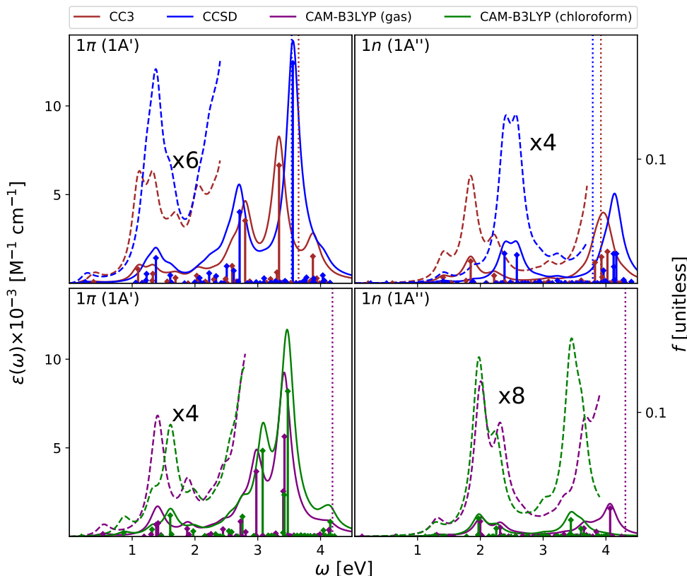
Fig. 3 Thymine. Upper panels : ESA at EOM-CCSD/aug-cc-pVDZ and EOM-CC3/aug-cc-pVDZ levels of theory in gas phase. Bottom panels : ESA at CAM-B3LYP/aug-cc-pVDZ level of theory in gas phase and in chloroform solution. The spectra in dashed line are enhanced by the factor given in the figures. Geometry optimized in the gas phase enforcing C_s symmetry. The vertical lines indicate the first ionisation energy in the gas phase (see Section 2 for details). HWHM = 0.0045563 Hartree.
