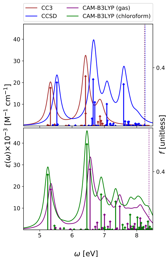
Fig. 6 Adenine. Upper panel : OPA at EOM-CCSD/aug-cc-pVDZ and EOM-CC3/aug-cc-pVDZ levels in gas phase. Bottom panel : OPA at CAM-B3LYP/aug-cc-pVDZ level of theory in gas phase and in chloroform solution. Geometry optimized in the gas phase enforcing C_s symmetry. The vertical lines indicate the first ionisation energy in the gas phase ( \Delta SCF at DFT level). Note that for CAM-B3LYP in gas phase the first intense peak is L_a , with n\pi^* almost overlapping with it. Then L_b follows. In solution, the first intense peak is L_a , followed by L_b and then by n\pi^* . HWHM = 0.0045563 Hartree.
