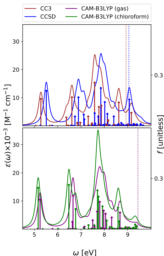
Fig. 2 Thymine. Upper panel : OPA at EOM-CCSD/aug-cc-pVDZ and EOM-CC3/aug-cc-pVDZ levels of theory in gas phase. Bottom panel : OPA at CAM-B3LYP/aug-cc-pVDZ level of theory in gas phase and in chloroform solution. Geometry optimized in the gas phase enforcing C_s symmetry. The vertical lines indicate the first ionisation energy in the gas phase ( \Delta SCF at DFT level). HWHM = 0.0045563 Hartree.
