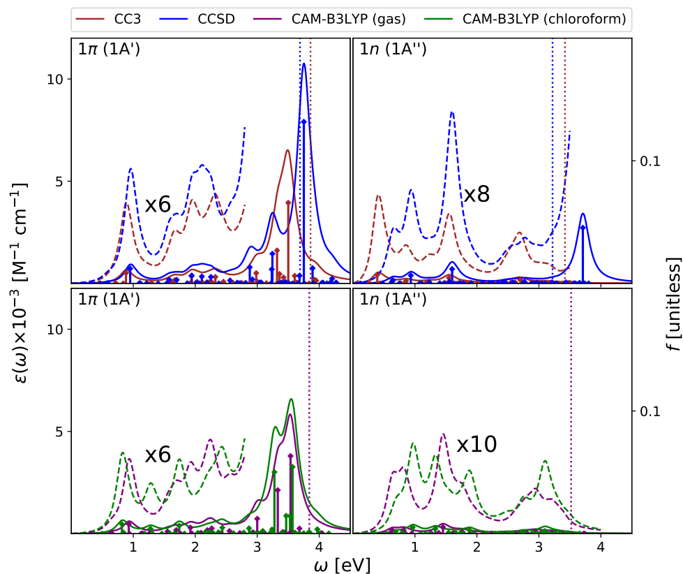
Fig. 5 Cytosine. Upper panels : ESA at EOM-CCSD/aug-cc-pVDZ and EOM-CC3/aug-cc-pVDZ levels of theory in gas phase. Bottom panels : ESA at TD-CAM-B3LYP/aug-cc-pVDZ level of theory in gas phase and in chloroform solution. The spectra in dashed line have been enhanced by the factor indicated. Geometry optimized in the gas phase enforcing C_s symmetry. The vertical lines indicate the first ionisation energy in the gas phase ( \Delta SCF at DFT level). HWHM = 0.0045563 Hartree.
