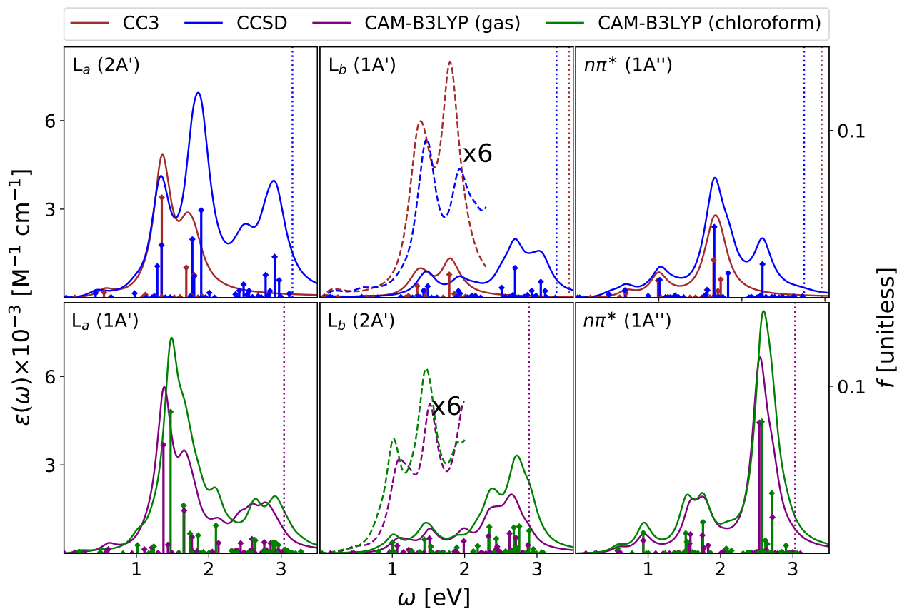
Fig. 7 Adenine. Upper panels : ESA at EOM-CCSD/aug-cc-pVDZ and EOM-CC3/aug-cc-pVDZ levels in gas phase. Bottom panels : ESA at CAM-B3LYP/aug-cc-pVDZ level of theory in gas phase and in chloroform solution. The spectra in dashed line were enhanced by the factors indicated in the figures. Geometry optimized in the gas phase enforcing C_s symmetry. The vertical lines indicate the first ionisation energy in the gas phase ( \Delta SCF at DFT level). It was assumed that EOM-CC3 provides the same order of states as EOM-CCSD. HWHM = 0.0045563 Hartree.
