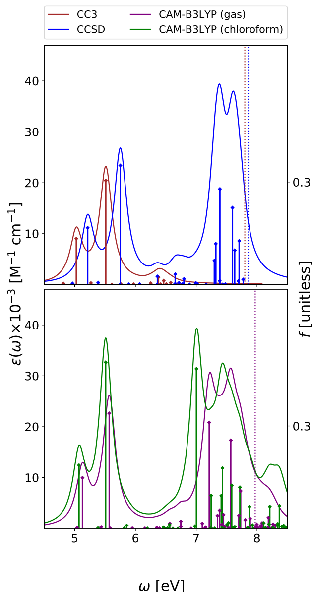
Fig. 8 Guanine. Upper panel : OPA at EOM-CCSD/aug-cc-pVDZ and EOM-CC3/aug-cc-pVDZ levels in gas phase. Bottom panel : OPA at CAM-B3LYP/aug-cc-pVDZ level of theory in gas phase and in chloroform solution. Geometry optimized in gas phase enforcing C_s symmetry. The vertical dashed lines indicate the first ionisation energy in the gas phase ( \Delta SCF at DFT level). HWHM = 0.0045563 Hartree.
