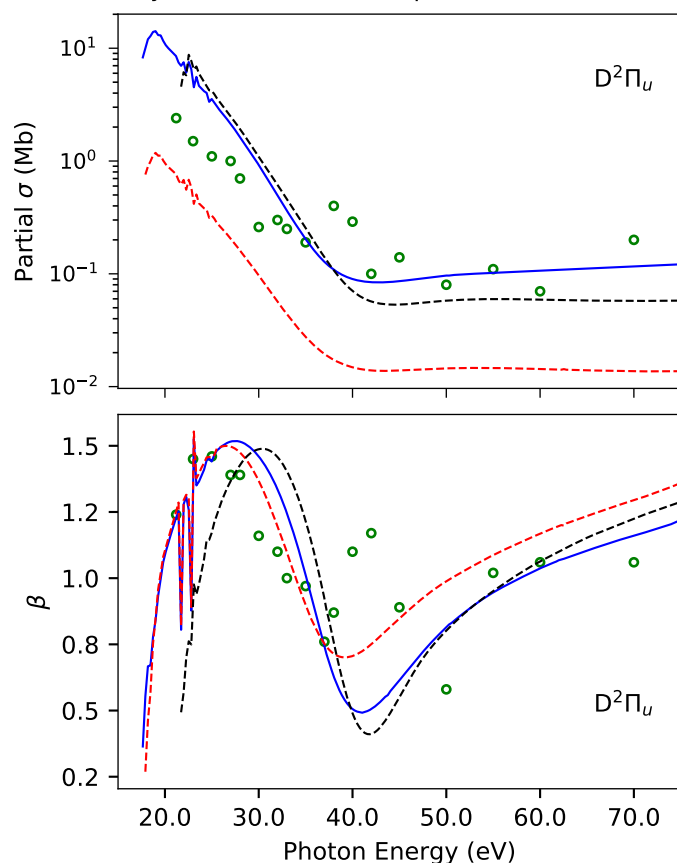
Fig. 6 CS 2 . Individual channel photoionization cross-section \sigma and asymmetry parameter \beta of the D band computed using B-spline TD-DFT continuum orbitals with Dyson orbitals computed using the aug-cc-pVDZ basis set. The experimental results (green dots) are from Ref. 96. The CCSD results were also reported in Ref. 45, together with CCSDR(3) corrected counterparts.
