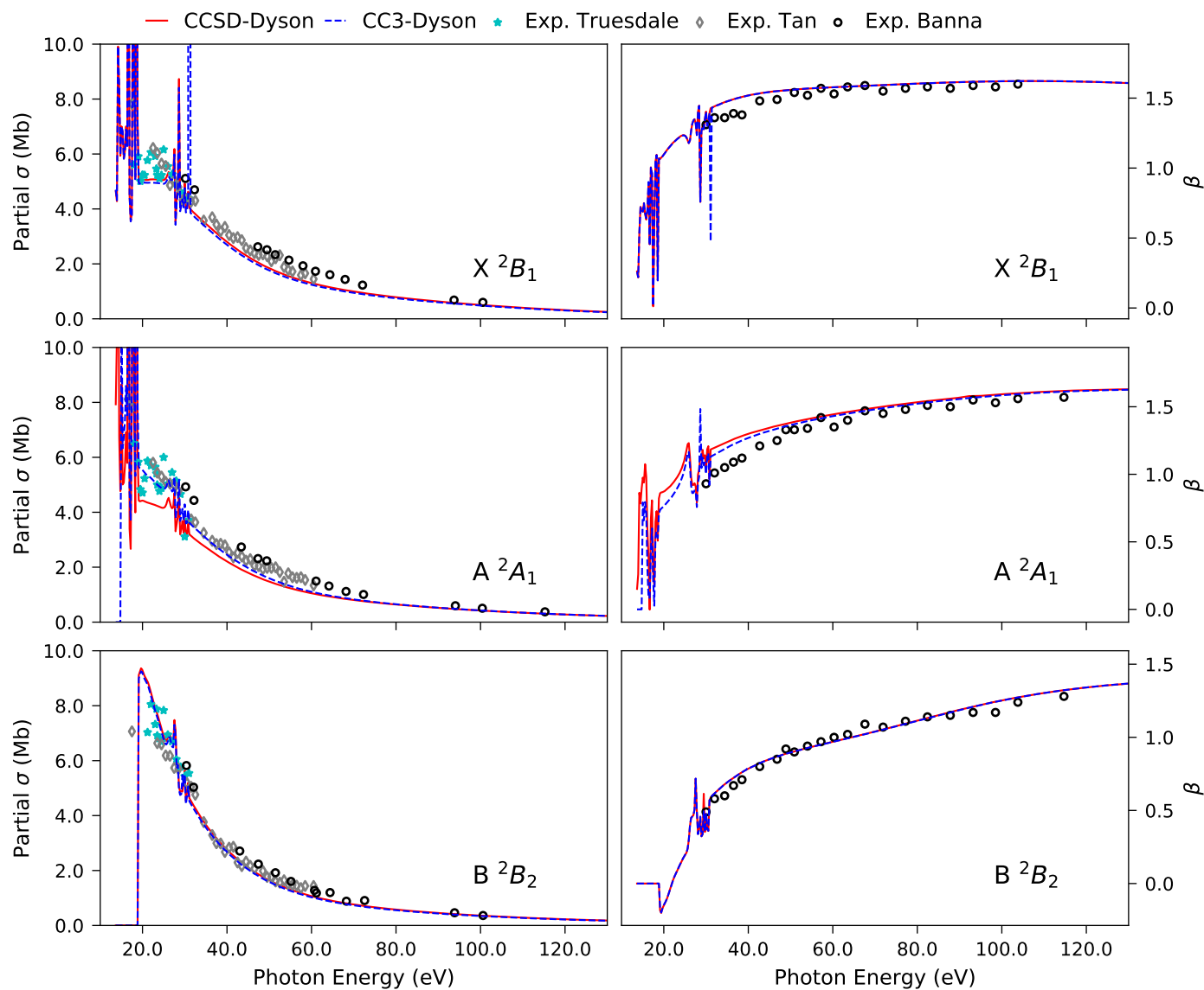
Fig. 2 \text{H}_2\text{O} . Partial cross-section \sigma (left panels) and asymmetry parameter \beta (right panels) for the primary ionization channels obtained using EOM-CCSD and EOM-CC3 Dyson orbital descriptions of the bound state. B-spline TD-DFT is used for the continuum orbital description. Experimental results are taken from Ref. 90–92.
