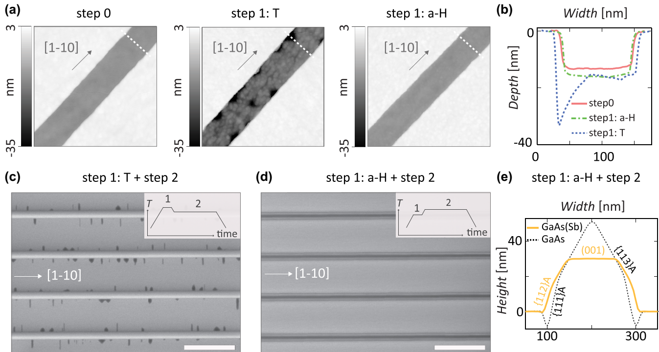
FIG. 2. (a) A set of AFM images ( 0.5 \times 0.5 \mu\text{m}^2 image size) demonstrating a [1\bar{1}0] -oriented GaAs growth window (trench) with a native oxide (step 0), after thermal oxide desorption (step 1: T), after atomic hydrogen oxide removal (step 1: a-H). White dashed lines indicate the position of AFM profiles shown in (b) and averaged over 15 nm. Top-view SEM images ( 1 \mu\text{m} scale bar) of GaAs(Sb) SAG nanowires grown on a GaAs(001) substrate from which the native oxide was removed either thermally (c) or with a-H (d). The insets show relative temperature T of oxide removal with respect to the GaAs(Sb) growth step with the latter being fixed at 600^\circ\text{C} . (e) AFM profile across a typical GaAs(Sb) SAG nanowire with step 1: a-H showing a faceted structure. AFM profile across a GaAs SAG nanowire grown without Sb surfactant but otherwise identical growth parameters is shown for comparison.
