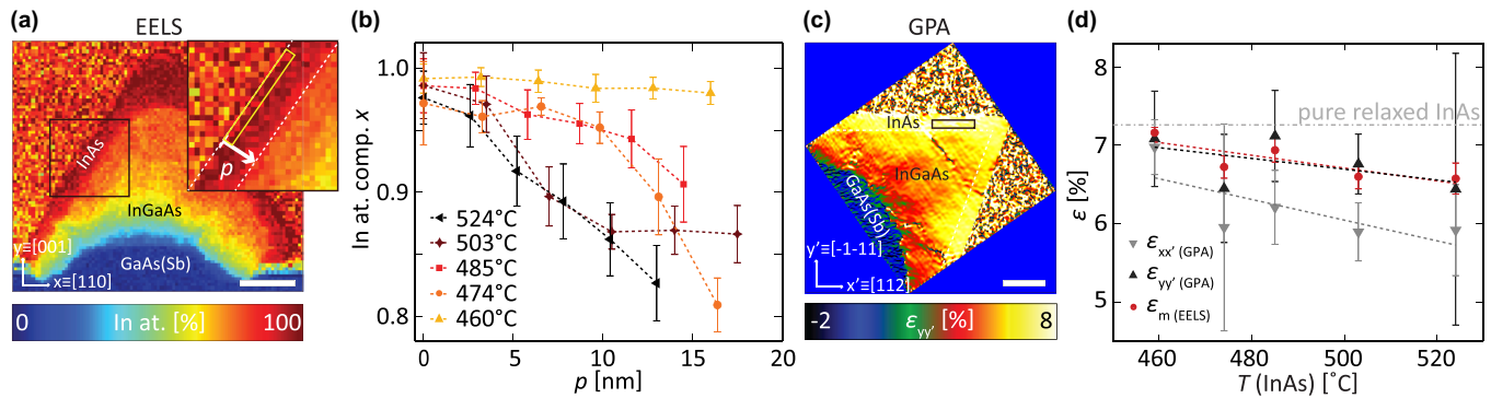
FIG. 4. Influence of the growth temperature on the InAs channel composition. (a) In atomic composition EELS map (relative to Ga; scale bar, 50 nm) of the sample with InAs channel grown at 485 °C. Inset: zoomed area of the channel indicating the procedure to obtain data points in (b). (b) In atomic composition x extracted at position p across the InAs channel grown at five different temperatures. For each growth temperature six data points are extracted. Each data point is taken at the position p and averaged over 100 nm [see inset in (a)]. The averaging gives the standard deviation as error bars. (c) An example of the out-of-plane lattice mismatch map ( \epsilon_{yy'} = \Delta d_{(\bar{1}\bar{1}1)}/d_{(\bar{1}\bar{1}1)} ) obtained with GPA (scale bar, 50 nm; GaAs is the reference) for the nanowire from (a). x axis is rotated 54.75° with respect to the original direction: x' = x + 54.75^\circ ( x' is parallel to the InAs/InGaAs interface, and thus to the [112] crystallographic orientation, y' is parallel to the [\bar{1}\bar{1}1] crystallographic orientation). (d) \epsilon_{yy'} and \epsilon_{xx'} as a function of the InAs growth temperature extracted from GPA. Each data point is averaged over a 50 \times 10 nm 2 box and presented with standard deviations as error bars. We also plot \epsilon_m calculated from the EELS composition assuming Vegard's law. In both cases, \epsilon increases with decreasing InAs growth temperature. The dashed lines are a linear fit to the experimental data and are guides to the eye.
