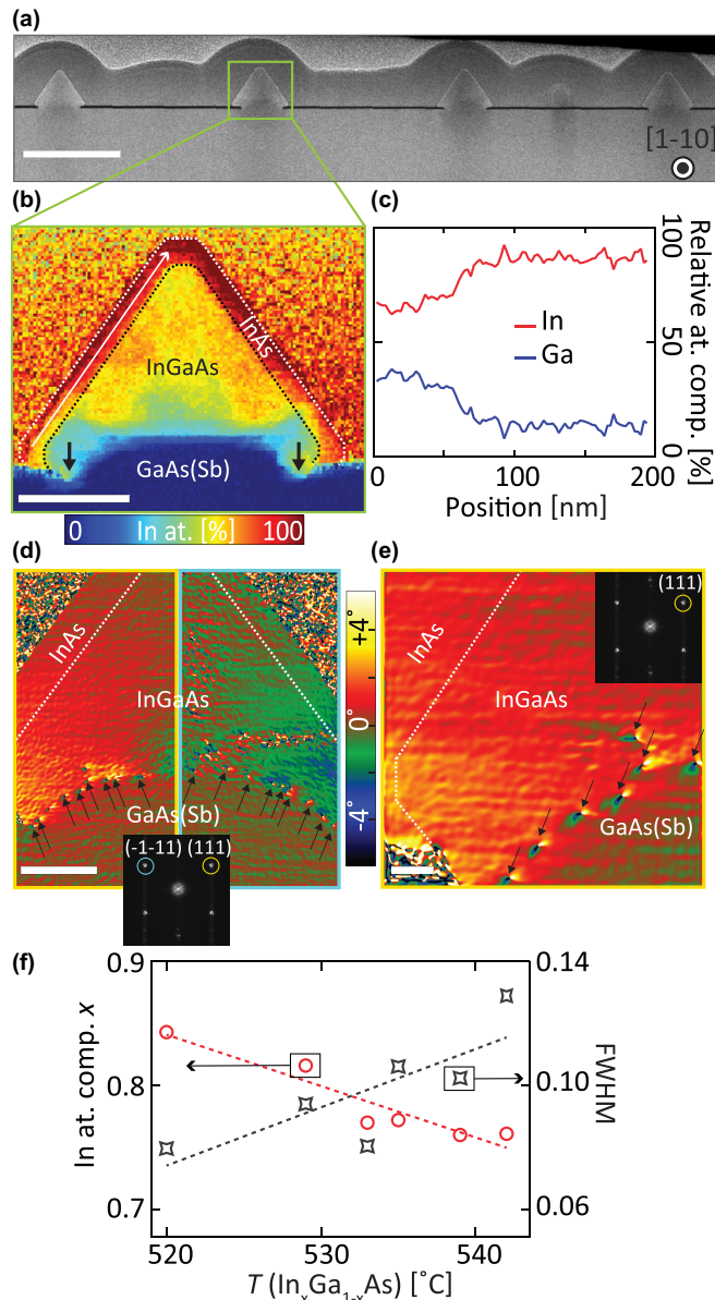
FIG. 3. The role of InGaAs growth temperature on the composition and crystal properties of the InAs/InGaAs/GaAs(Sb) SAG nanowires. (a) Low magnification HAADF-STEM image (scale bar, 500 nm) of a lamella taken across [1\bar{1}0] -oriented field-effect nanowires grown at 522 °C. (b) In atomic distribution EELS map (relative to Ga, in atomic percentage; scale bar, 100 nm) of the nanowire from (a). Arrows indicate the place of erosion of GaAs(Sb) and GaAs. (c) Relative Ga and In atomic composition profile along the (\bar{1}\bar{1}1) facet in the InAs channel from (b). [(d),(e)] GPA rotational maps of the nanowire from (b) representing its central part (50 nm scale bar) and the left corner (10 nm scale bar). Misfit dislocations at the InGaAs/GaAs(Sb) buffers are highlighted with black arrows. The insets show the corresponding fast Fourier transform (FFT) with the analysed planes: (111) planes correspond to the left half and (\bar{1}\bar{1}1) planes to the right half of the image in (d). (f) x in the buffer as a function of the buffer growth temperature T extracted from XRD reciprocal space maps. The peak broadening representative of the compositional variations in the buffer measured as FWHM is plotted as well. The dashed lines are linear fits and are guides to the eye.
