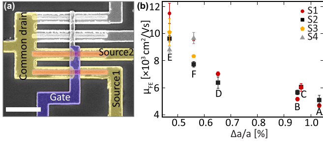
FIG. 5. The role of the InAs/InGaAs interface quality on the electrical properties of InAs/InGaAs/GaAs(Sb) nanowires. (a) False-colored SEM image of field-effect devices (2 \mu\text{m} scale bar). Measured nanowires appear in red, Au/Ti contacts (in yellow), the top Au/Ti gate (in violet). (b) Electron mobility \mu_{FE} as a function of the InAs/InGaAs lattice mismatch, \Delta a/a , for six samples collected in Table I: A–F. Two nanowires per sample for samples A–D are measured: S1 and S2 both having 500-nm channel length [corresponding to Source 1 and Source 2 in (a)] and four nanowires per sample for samples E and F are measured: S1, S2, S3, S4, all having 500-nm channel length.
