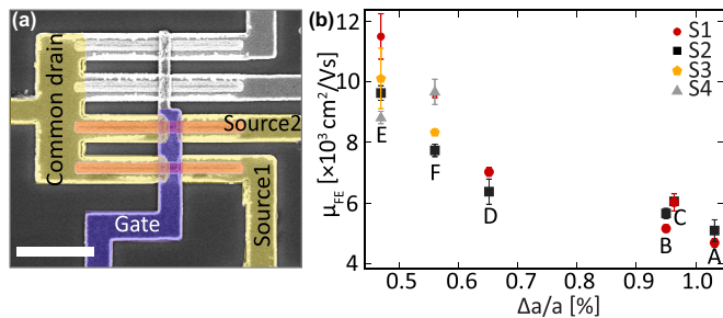
FIG. 5. The role of the InAs/InGaAs interface quality on the electrical properties of InAs/InGaAs/GaAs(Sb) nanowires. (a) False-colored SEM image of field-effect devices (2 \mu m scale bar). Measured nanowires appear in red, Au/Ti contacts (in yellow), the top Au/Ti gate (in violet). (b) Electron mobility \mu_{FE} as a function of the InAs/InGaAs lattice mismatch, \Delta a/a , for six samples collected in Table I: A–F. Two nanowires per sample for samples A–D are measured: S1 and S2 both having 500-nm channel length [corresponding to Source 1 and Source 2 in (a)] and four nanowires per sample for samples E and F are measured: S1, S2, S3, S4, all having 500-nm channel length.
