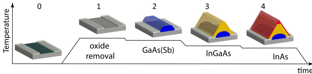
FIG. 1. Schematics of growth steps of InAs/InGaAs/GaAs(Sb) SAG nanowires on GaAs(001) substrates covered with a 10-nm thick SiO 2 mask. 0. Substrate fabrication; 1. Native oxide removal; 2. GaAs(Sb), 3. InGaAs and 4. InAs layer growth. Note that the originally faceted GaAs(Sb) buffer becomes rounded after the growth of InGaAs and InAs layers on top.
