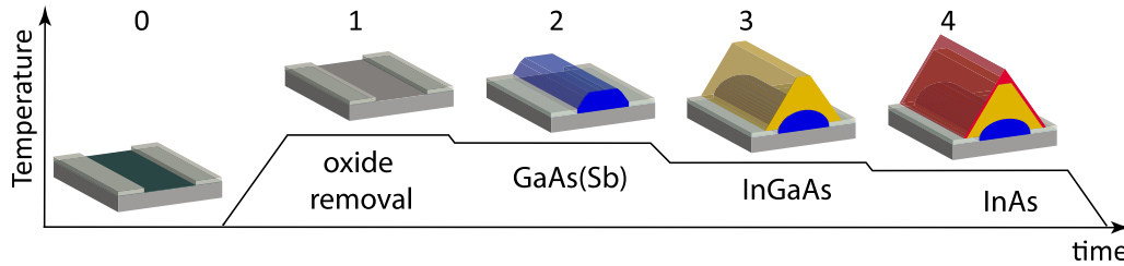
FIG. 1. Schematics of growth steps of InAs/InGaAs/GaAs(Sb) SAG nanowires on GaAs(001) substrates covered with a 10-nm thick \text{SiO}_2 mask. 0. Substrate fabrication; 1. Native oxide removal; 2. GaAs(Sb), 3. InGaAs and 4. InAs layer growth. Note that the originally faceted GaAs(Sb) buffer becomes rounded after the growth of InGaAs and InAs layers on top.
