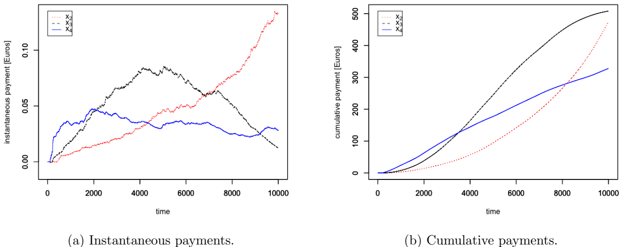
Figure 4: Temporal evolution of the payments (instantaneous and cumulative) for the various features of the support agents over the period considered. These results are for a nominal level \tau = 0.9 .
