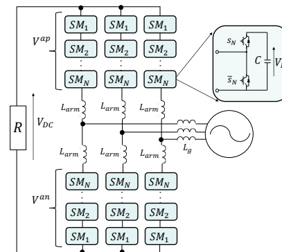
Fig. 2. Circuit topology of the three-phase MMC considered in this work.
