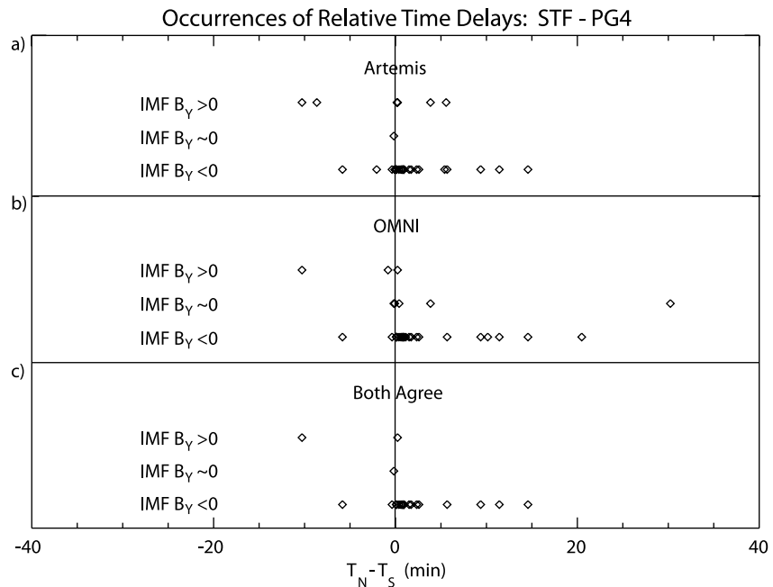
Figure 9. Plots of the distribution of time delays ( T_N - T_S ) between observations of the \Delta Bx minima associated with each GMD event in at the STF-PG4 station pair. Panel (a) shows events with interplanetary magnetic field (IMF) B_y > 1 , within \pm 1 of 0, and < -1 , respectively, as measured by Artemis/Themis. Panel (b) shows events measured by OMNI, and panel (c) shows only those events for which Artemis/Themis and OMNI IMF categories agreed.
