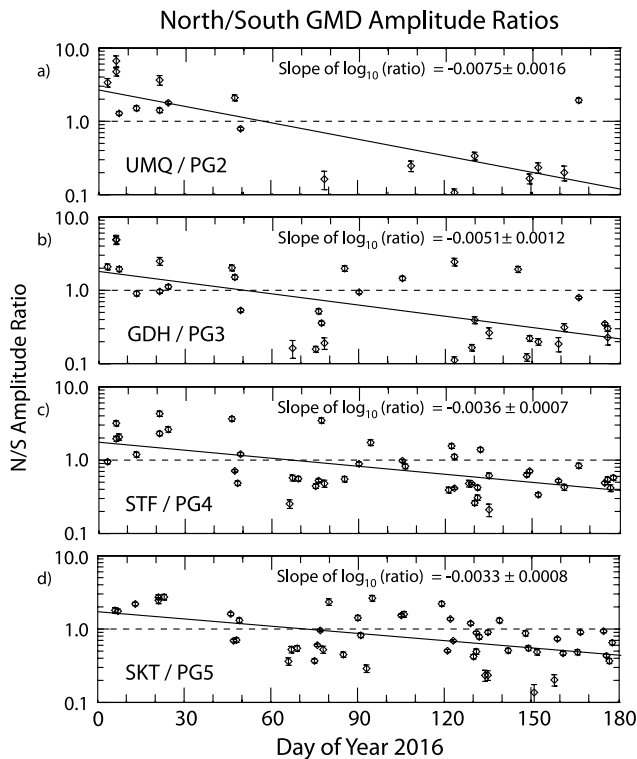
Figure 7. Plot of the ratio of GMD derivatives at northern and southern stations, \frac{dB_N}{dt}/\frac{dB_S}{dt} , as a function of the day of the year in 2016 for each of the four conjugate station pairs: (a) UMQ/PG2, (b) GDH/PG3, (c) STF/PG4, and (d) SKT/PG5. Only those events with at least one >6 nT/s event at each station pair are shown.
