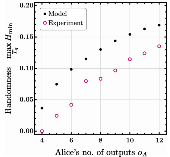
FIG. 3. Results obtained from experimental data of Ref. [42]. Min-entropy vs Alice's number of outputs. The optimal values of H_{\min} from the idealized theoretical model (black dots) and the lower bounds on H_{\min} from the experimental data (pink circles) are pictured. Alice and Bob both measure q and p , and randomness is extracted from Alice's q measurement. H_{\min} is maximized over Alice's binning period in the range T_q \in [2, 10] . Bob has o_B = 16 outcomes.
