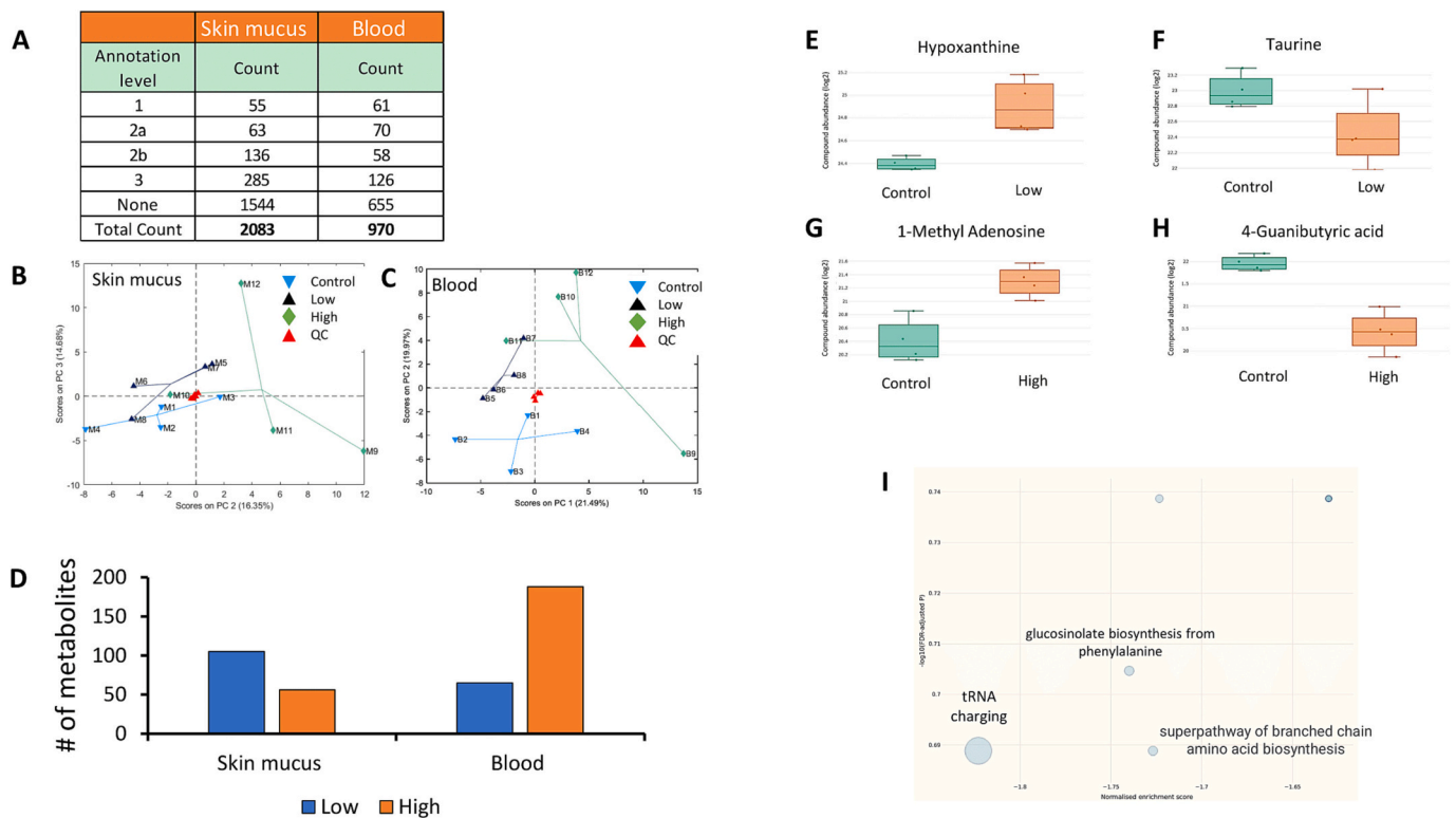
Fig. 7. Metabolomic changes in the skin mucus and blood of Atlantic salmon transiently exposed to H_2S . A ) The total number of compounds identified. B, C ) Score plot from PCA model calculated on the relative concentrations of the variables in the reduced dataset of B ) skin mucus and C ) blood metabolome. Data have been auto-scaled. D ) Number of metabolites that significantly changed following transient exposure to H_2S relative to the unexposed control group. Representatives from level 1 metabolites significantly changed in (E, F) skin mucus and (G, H) blood. Only the representative metabolites from the low group are given in the skin mucus, while only those from the high group are in the blood based on the dose profile in D . I ) Plot of statistical significance of pathway-specific gene set enrichment ( -\log_{10} FDR-adjusted p -value) against normalised enrichment score (NES). The size of each point reflects the number of compounds evaluated for each pathway. Only pathways with P (FDR) < 0.25 were included.
