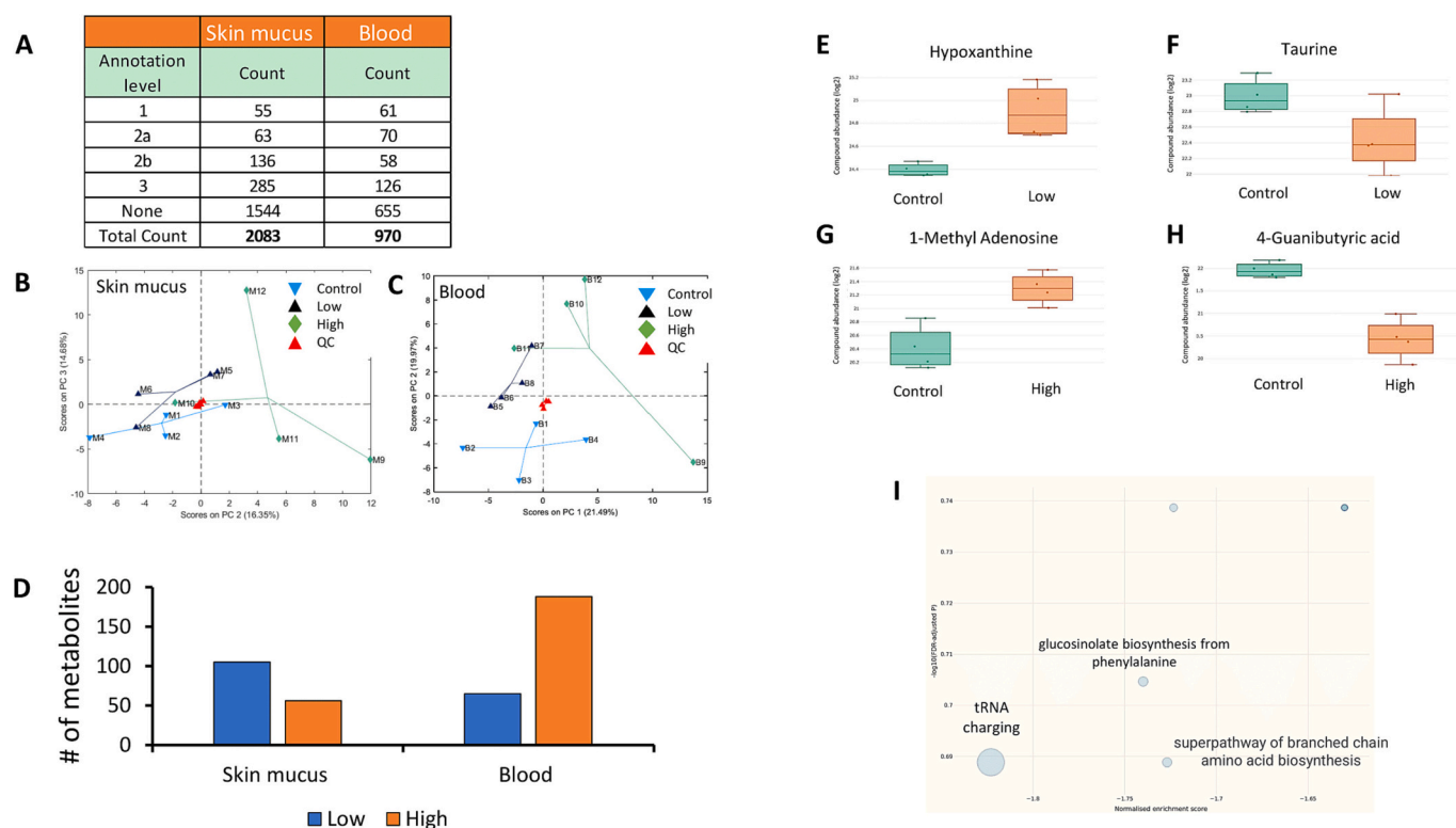
Fig. 7. Metabolomic changes in the skin mucus and blood of Atlantic salmon transiently exposed to H_2S . A) The total number of compounds identified. B, C) Score plot from PCA model calculated on the relative concentrations of the variables in the reduced dataset of B) skin mucus and C) blood metabolome. Data have been auto-scaled. D) Number of metabolites that significantly changed following transient exposure to H_2S relative to the unexposed control group. Representatives from level 1 metabolites significantly changed in (E, F) skin mucus and (G, H) blood. Only the representative metabolites from the low group are given in the skin mucus, while only those from the high group are in the blood based on the dose profile in D . I) Plot of statistical significance of pathway-specific gene set enrichment ( -\log_{10} FDR-adjusted p -value) against normalised enrichment score (NES). The size of each point reflects the number of compounds evaluated for each pathway. Only pathways with P (FDR) < 0.25 were included.
