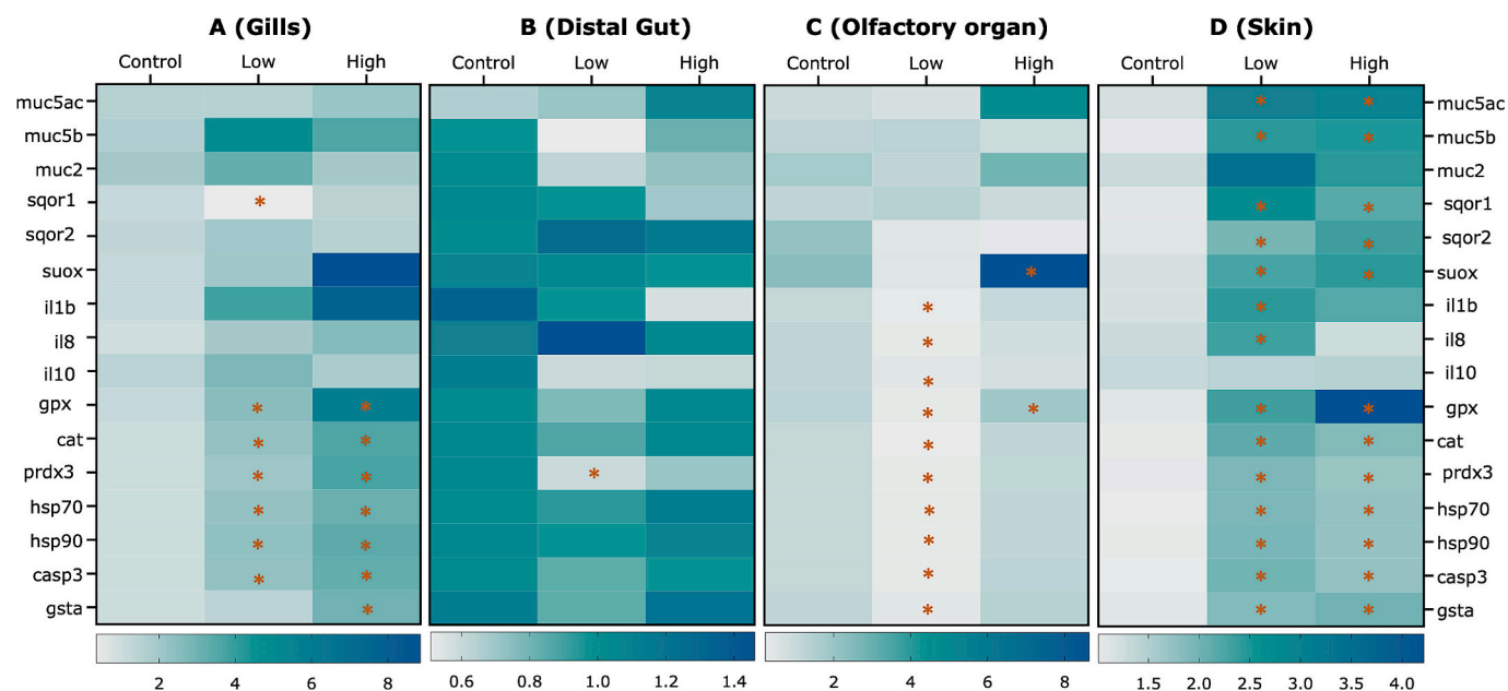
Fig. 2. Gene expression profiles in (A) gills, (B) distal gut, (C) olfactory organ, and (D) skin of Atlantic salmon transiently exposed to different H 2 S levels for 1 h: control (0 μM), low (0.6 μM), and high (1.2 μM). The gradients indicate a mean of n = 8 ; stars denote a statistically significant difference from the control ( p -value < 0.05) inferred by pairwise comparison.
