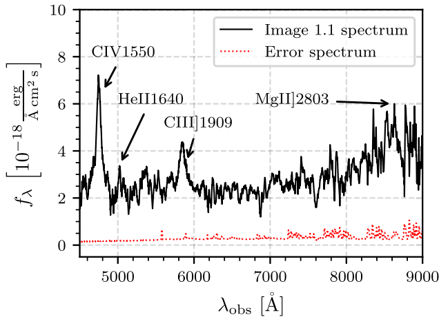
Figure 4. LDSS3 spectrum of image 1.1 (black) and its 1\sigma uncertainty (red), which was published in Mainali (2019). The two prominent broad emission lines are identified as the C IV \lambda 1550 \text{ \AA} and C III \lambda 1909 \text{ \AA} (unresolved) doublets at z_{\text{spec}} = 2.063 \pm 0.005 . There is also a He II \lambda 1640 \text{ \AA} detection and a hint at the Mg II \lambda 2803 \text{ \AA} doublet towards the high-wavelength end.
