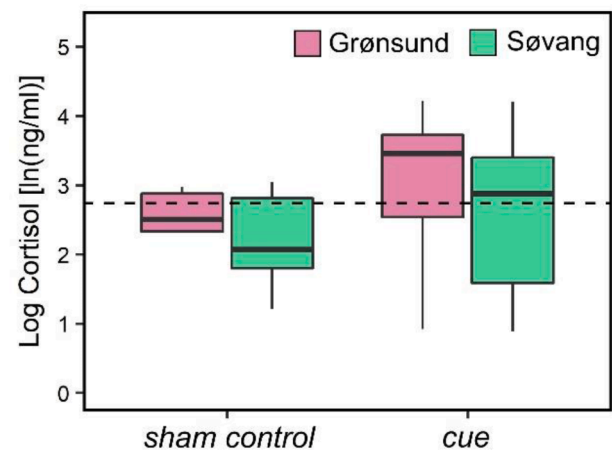
Fig. 4. Blood cortisol response to a chemical alarm cue. The dotted line represents the baseline measurements for cortisol in the baseline control treatment group. Concentrations are significantly higher in the cue treatment group, but there is no difference between populations. In boxplots horizontal bars, boxes and vertical lines represent the median, interquartile range, non-outlier range, respectively.
