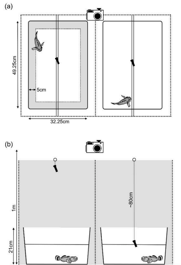
Fig. 2. Behavioural arenas (a) aerial view, and (b) front view. In (a), the grey area represents the 5 cm edge zone used to measure centre area use behaviour, and the parallel lines across the arenas represent the clear acrylic tube used to suspend the bolt above the centre of the arena. The fishing line runs through the length of the tube and can be released and retracted by the observer. The bolt-release mechanism sits on top of a frame used to hold the polystyrene walls around the arena (dotted lines), and to hold the camera in position, so that the bolt drops approximately 80 cm to break the water surface before retraction.
