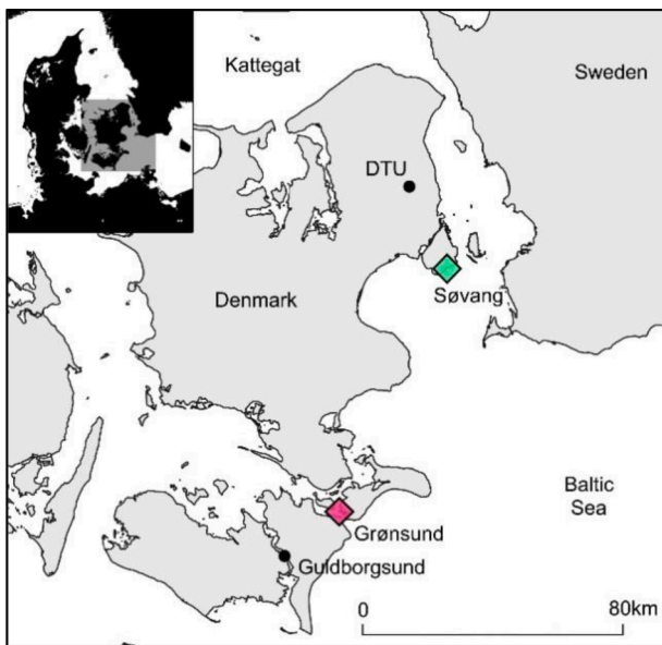
Fig. 1. Study sites in on the eastern coast of Denmark, and inset, within the broader south-east Baltic Sea region. Round gobies were first recorded in the areas around Grønsund (pink) and Søvang (green) in approximately 2011 and 2016, respectively, 10 and 5 years prior to sampling. Grønsund is located directly north of Guldborgsund, the first area of inner Danish waters invaded by round gobies in 2009. Søvang is located just south of Copenhagen, nearer to the DTU Lyngby laboratory in northern Copenhagen. At present, DTU Lyngby is approximately level with the northern edge of the round goby's invasion front up the eastern coast of Denmark.
