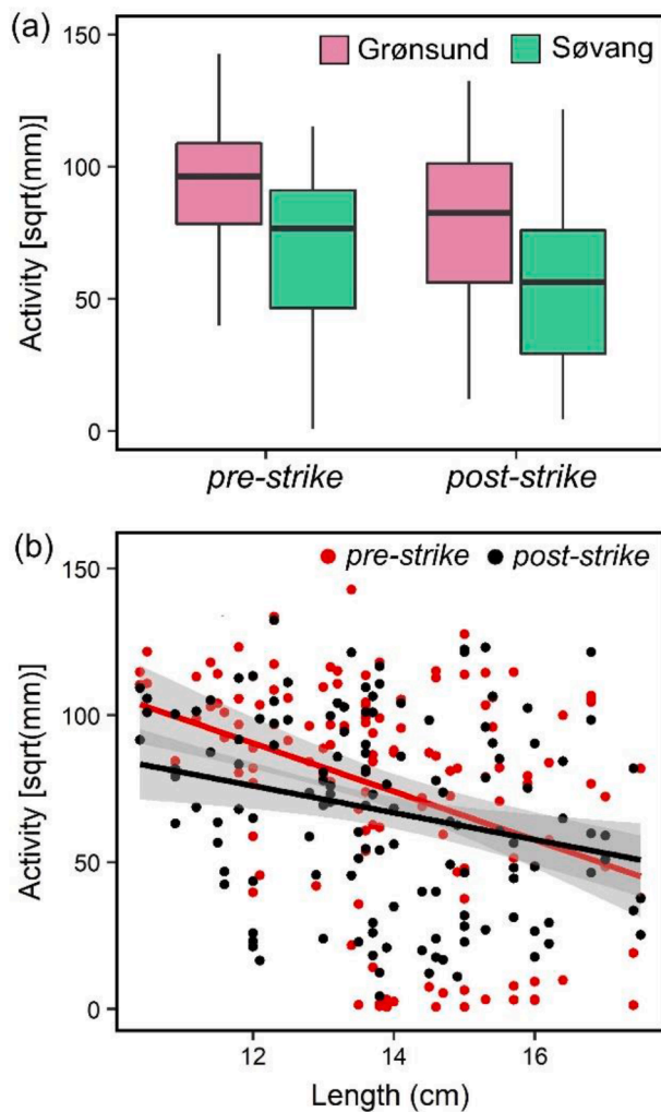
Fig. 3. Activity response in Experiment 1, associated with (a) population, and (b) SL. In (a) fish from the newer site Søvang (est. 2016) appear to reduce their activity levels following the predator cue more than Grønsund (est. 2011) fish. In (b) smaller fish were more active overall but reduced their activity levels more relative to larger fish following the predator cue. In boxplots horizontal bars, boxes and vertical lines represent the median, interquartile range, non-outlier range, respectively.
