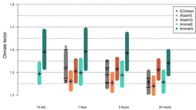
Fig. 5. Annual CFs for the 2-year return level and durations 15 min, 1 h, 3 h and 24 h. Bars represent the spatial interquartile range with the median marked as a plus sign. For the EC-ensemble (grey) bars represent the field interquartile range of the ensemble, while black lines represent the 25th and 75th percentile of the 21 model means.
