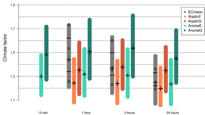
Fig. 6. Similar to Fig. 5, for annual CFs for the 100-year return level and durations 15 min, 1 h, 3 h and 24 h.
