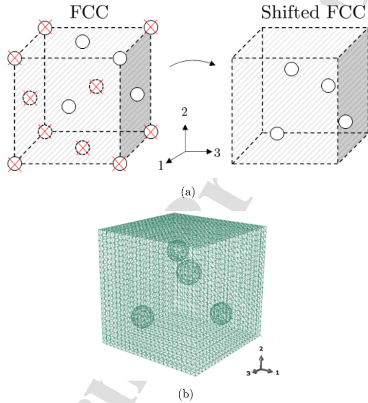
Figure 3: Procedure for modeling a Face-Centered Configuration (FCC) of the voided unit cell, showing (a) the FCC unit cell where the voids removed (left) are outside the shifted unit cell (right), and (b) the corresponding finite element mesh of the FCC unit cell.
