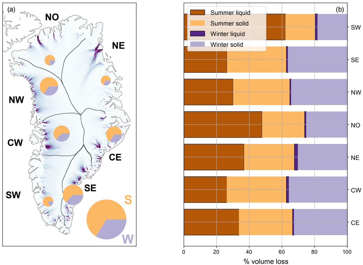
Fig. 3 Seasonality of all regions in Greenland. (a) Summer (brown) and winter (purple) volume loss for each region where the size of the circles indicates the total volume loss. The background image shows ice-flow velocities from MEaSURES (Joughin 2020). (b) Same as (a) but as bars. The proportion of the volume loss that is liquid is shown with darker colours and a black outline. The seven regions are defined by Mouginot et al. 2019c as follows: south-west (SW), central west (CW), north-west (NW), north (NO), north-east (NE), central east (CE), and south-east (SE).
