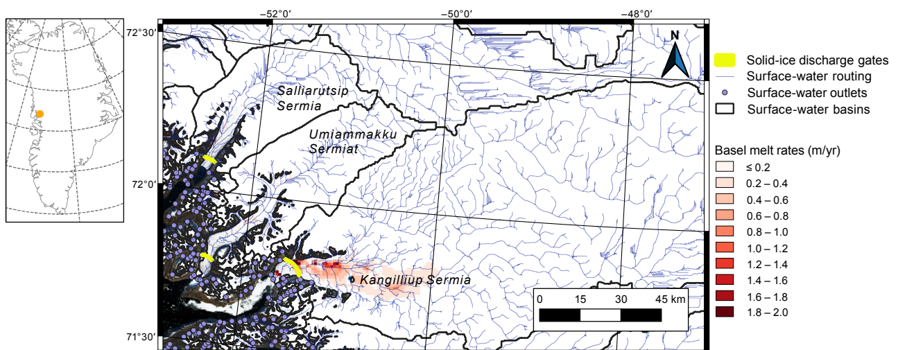
Fig. 1 Example from West Greenland showing the three data products. Yellow lines indicate the locations of solid-ice discharge gates from M2020. The surface-meltwater product is shown as blue streamlines with water outlets as purple dots and their associated basins in black . The basal-melt product is shown in red as \text{m/yr} . Background image from Satellite background image is from Sentinel-2 (European Space Agency), 20 August 2022.
