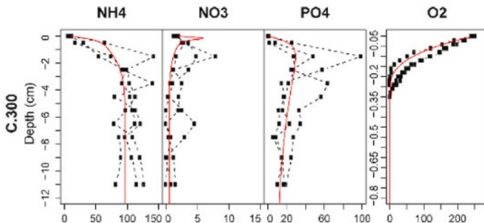
Figure 52. Examples of porewater nutrient profiles data used to parameterize OMEXDIA (De Borger et al. , 2021b).
