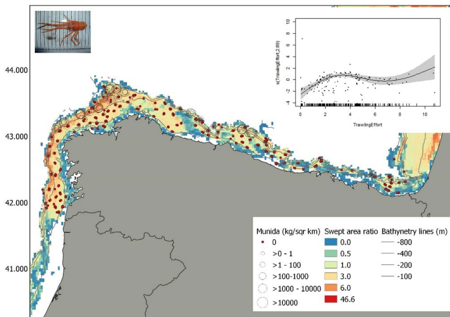
Figure 45. Distribution of swept are ration and Munida spp. abundance in the northern coast of Spain and response curve for trawling effort and Munida spp abundance. The curve shows a clear positive effect of trawling on Munida abundance in the first levels of trawling (from 0 to 3) with a less clear trend after these values.
