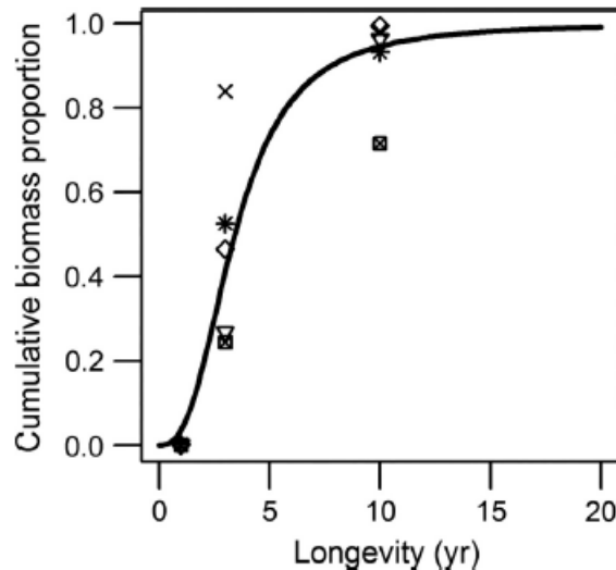
Figure 62. An example of the cumulative biomass–longevity relationship estimated from the observed cumulative biomass by longevity class (1, 1–3, 3–10 yr) in five sampling stations. Different symbols indicate the five different locations. Figure taken from Rijnsdorp et al. (2018).
