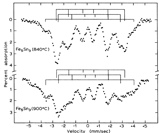
FIG. 4. \text{Fe}^{57} Mössbauer spectra at 300 °K for the high- and low-temperature modifications of \text{Fe}_5\text{Sn}_3 . The subdivision into three separate components was decided on the basis of several spectra obtained at different temperatures.
