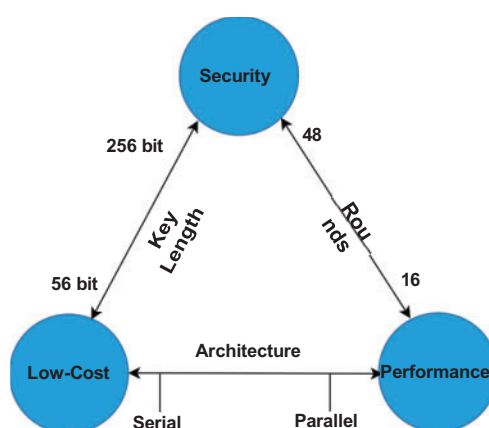
Figure 6: Design tradeoffs for lightweight cryptography system
