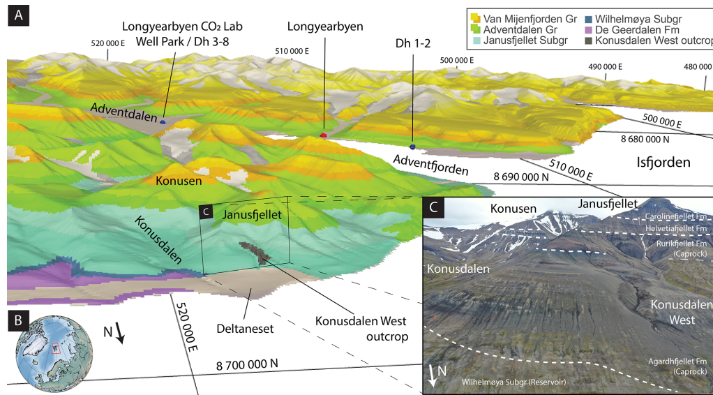
Figure 1. Location and geology of the Longyearbyen CO 2 Lab reservoir, cap rock, and overburden successions in Svalbard ( b ). The locations of the outcropping Konusdalen West exposures at Deltaneset and the city of Longyearbyen, and both drill sites of the Longyearbyen CO 2 Lab are highlighted ( a ). The inset ( c ) shows an overview photo of the study area. Geological map (1 : 250 000) and digital terrain model (50 m resolution) are courtesy of Norwegian Polar Institute (2014) and Norwegian Polar Institute (2016), respectively. The grid uses the WGS 84/UTM Zone 33N (EPSG:32633) projection.
