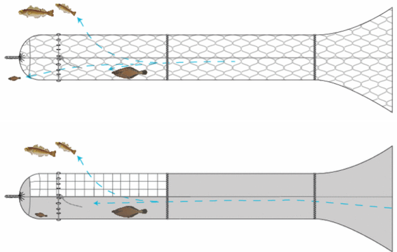
Figure 33. T90 (upper) and Bacoma (lower) codends © Thünen Institut.
