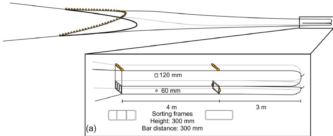
Figure 30. A conceptual drawing of the horizontally divided codend used as one of the codends in the twin-rig of the trawler in the winter.
