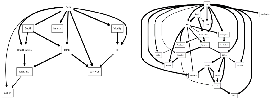
Figure 63. The consensus causal networks computed by taking the most frequent arcs appearing in the 200 networks learned, without (left) and with (right) the individual reflexes and injuries.
