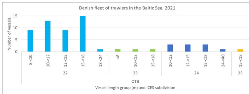
Figure 14. Distribution of the OTB fleet (n = 61) in 2021 given for each vessel length group in subdivisions 22-25; the vessels were allocated to the area in which they have conducted most of their trips.
