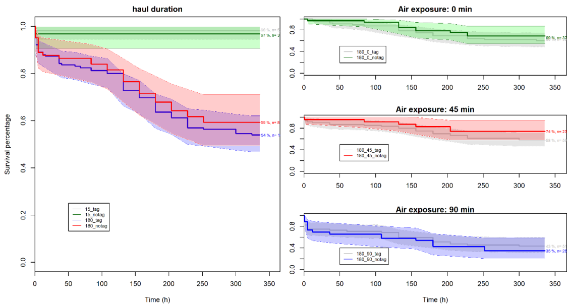
Figure 27. Kaplan Meier survival curves for plaice.
