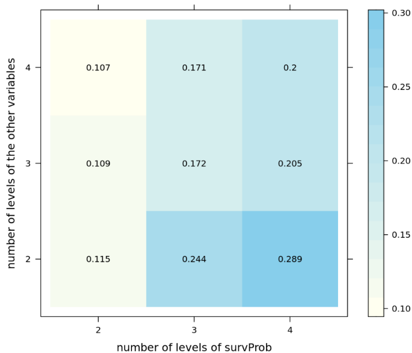
Figure 62. Classification error for different number of levels of response (survival probability “survProb”) and explanatory variables in the Bayes models.
