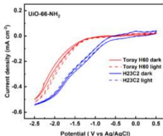
Figure 3. On-off CV curves at 50 \text{ mV s}^{-1} of UiO-66-NH 2 with hydrophobic carbon support layers in EC configuration and PEC configuration under dark and light irradiation.
