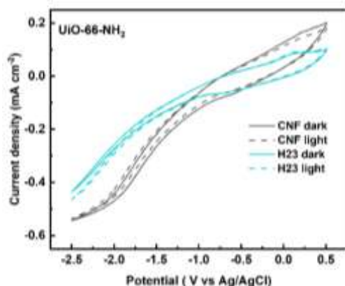
Figure 2. On-off cyclic voltammetry (CV) curves at 50 \text{ mV s}^{-1} of UiO-66-NH 2 with hydrophilic carbon support layers in PEC configuration under dark and light irradiation.
