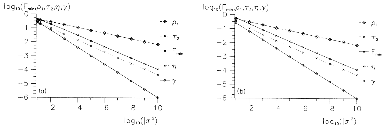
FIG. 3. Minimized Fano factor and optimized system parameters as a function of input photon number |\sigma|^2 . (a) Numerical optimization, (b) “approximate” optimization.
