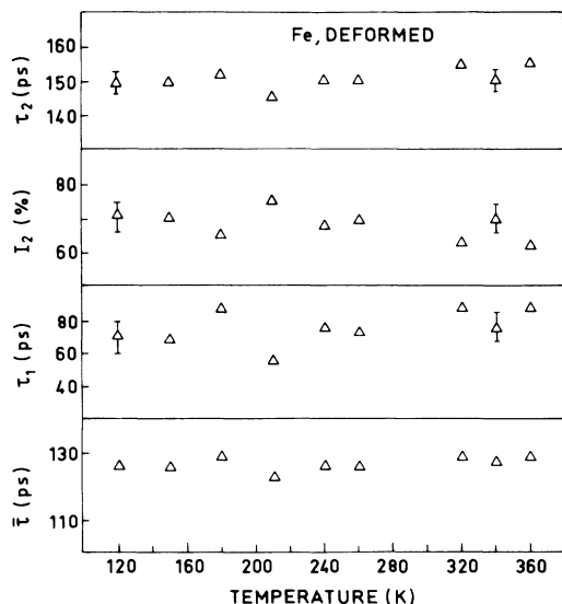
FIG. 7. Positron-annihilation parameters as a function of temperature for iron deformed at 77 K.
