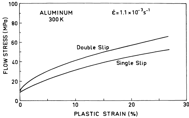
FIG. 2. Stress-strain curves at room temperature for aluminum single crystals initially oriented for single and double slip.
