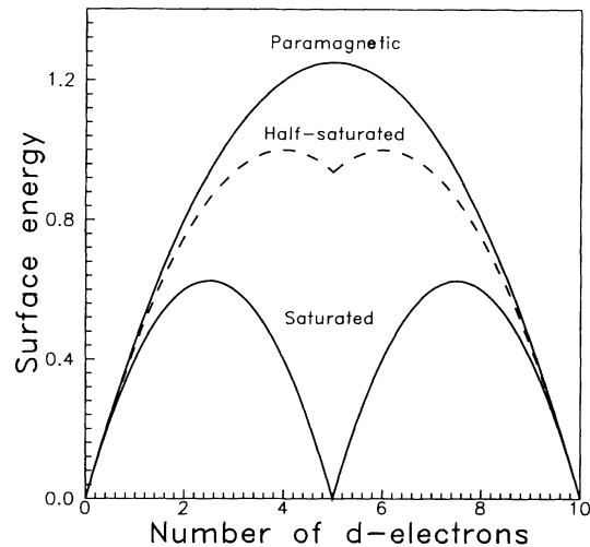
FIG. 2. Models of the surface energy of the 3d transition metals based on a constant d state density. The three curves correspond to the paramagnetic, the half-saturated, and the saturated cases described in the text.
