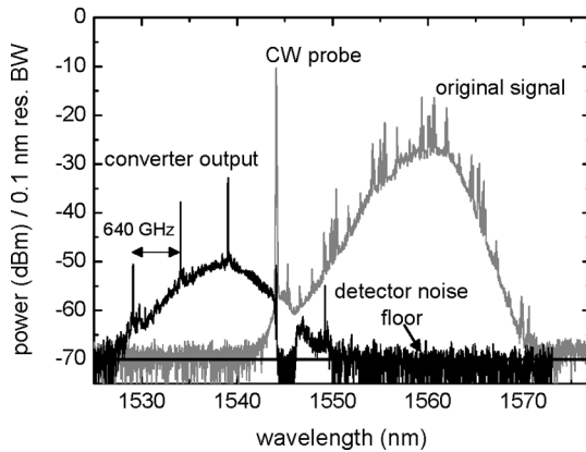
Fig. 7. Optical spectra illustrating the wavelength conversion process. The original signal along with the CW probe at the input to the HNFL is shown in the gray line. The output of the HNFL after filtering is shown in the black line. This is the spectrum of the wavelength-converted signal.
