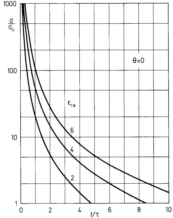
Figure 1. Temporal variation of the surface charge density \sigma at the time-zero charge location.
