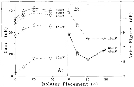
Fig. 2. Measured gain and noise figure versus the relative isolator placement between 0 and 50% of the total fiber length. Shown for pump power levels between 10 and 60 mW.
