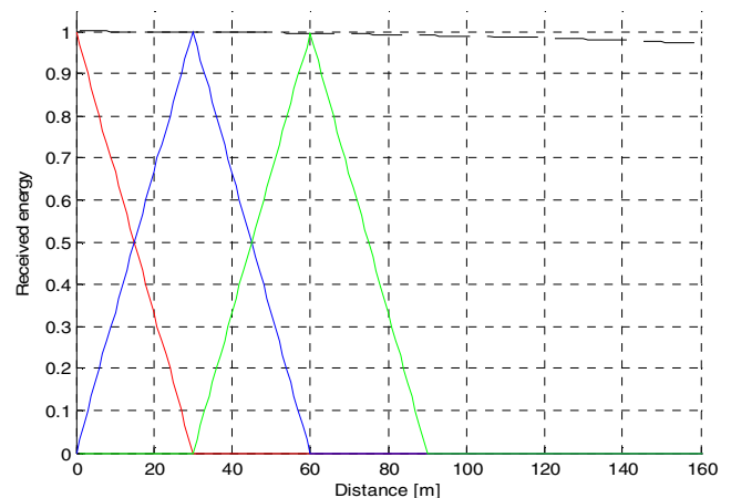
Figure 5: Normalized received energy profiles of the three first range cells of an undelayed collimated FSPT modulated lidar. Range cell one in red, two in blue and three in green. The dashed black line outlines W_{\text{collimated}}(x) .
