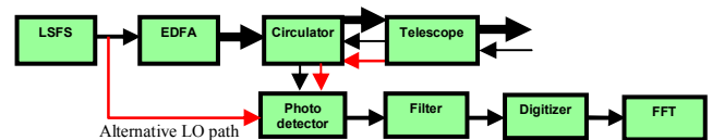
Figure 4: Layout of an FSPT modulated coherent monostatic lidar. LO in red.
