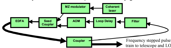
Figure 3: LSFS concept for generating FSPTs.
