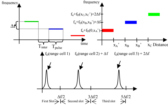
Figure 1 a) An FSPT with pulse duration, T_{pulse} , interpulse duration, T_{inter} , and pulse-to-pulse frequency step, \Delta f . b) Frequency as a function of scattered distance received by the lidar at time t_a when a full pulse has just been emitted. Note that the ranges contributing at t_a are x_A' = (c/2)(T_{pulse}) , x_B = (c/2)(T_{pulse} + T_{inter}) and x_B' = (c/2)(2T_{pulse} + T_{inter}) etc. c) The scatter from the first three range cells mapped into their allocated frequency slots, f_{offset} = 0 MHz in this case.
