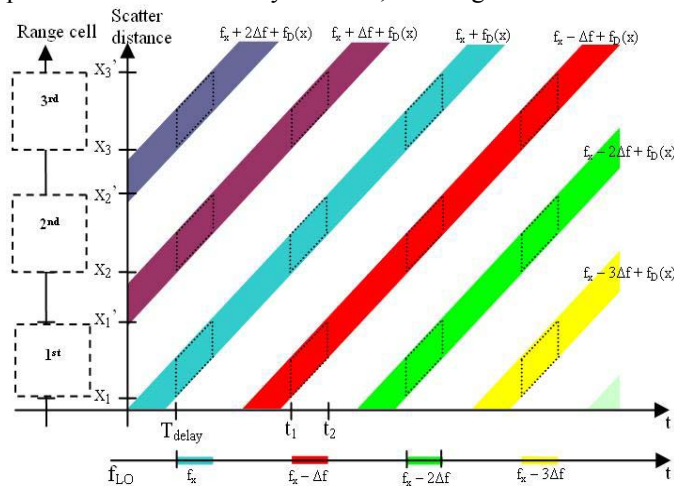
Figure 2: Time-space representation of scatter detected by an FSPT modulated lidar with a delayed LO and a considerable inter pulse duration for clarity.
