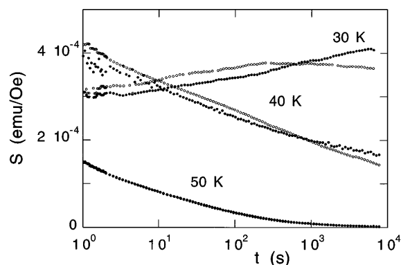
FIG. 4. Relaxation rate S vs time at the temperatures 30, 40, and 50 K for the 5 vol % sample. The wait time t_w at constant temperature before applying the probe field was 10^2 s (open symbols) and 10^4 s (filled symbols).
