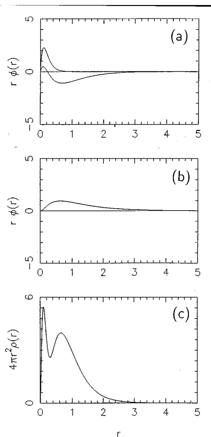
FIG. 2. Orbitals and total electron density for a Ne atom. (a) and (b) show rR_n(r) for (a) s functions and (b) p functions, and (c) shows 4\pi r^2 \rho(r) .
