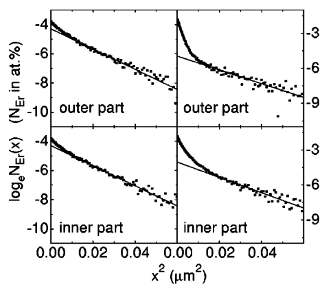
FIG. 1. Erbium concentration SIMS profiles for samples having different initial dopant levels: 0.1 at. % (left) and 0.4 at. % (right). Both samples annealed 21 h at 1100 °C. Inner and outer part are the tail closest to and the one farthest away from the silicon substrate, respectively. A straight line, which corresponds to a Gaussian profile in this representation, has been fitted to the low concentration part of each profile ( N_{\text{Er}} \leq 0.01 at. %).
