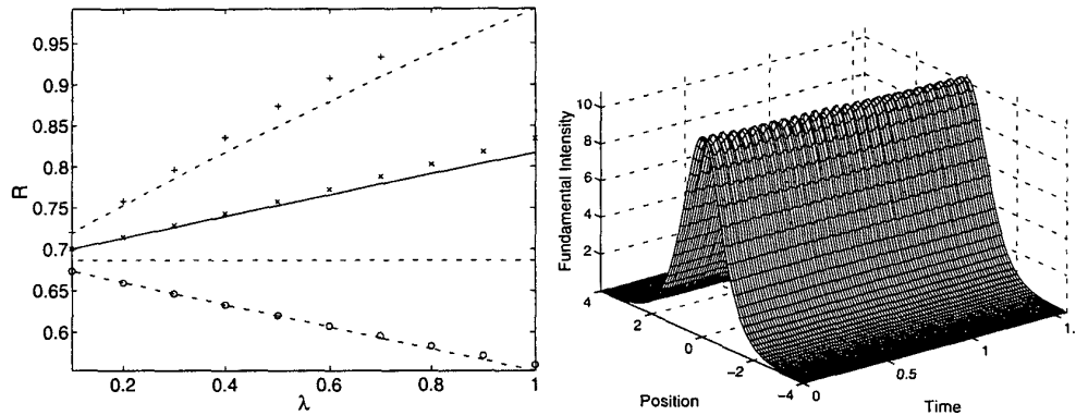
Fig. 2. LEFT: Ratio of peak intensities R = \bar{v}^2(0)/\bar{w}^2(0) versus the soliton parameter \lambda , calculated from the first-order solutions with \tilde{\gamma} = 0.0189 (solid), \tilde{\gamma} = 0.0474 (dot-dashed) and \tilde{\gamma} = -0.0189 (dashed), and from the zeroth-order solution ( \tilde{\gamma} = 0 , dotted). The ratios were also calculated from the average of the evolving field solutions for K = 10 (crosses), K = 4 (pluses) and K = -10 (circles). In all cases, \beta = 0 . RIGHT: Cubic (sech) bright soliton propagation in the dual grating, showing the evolution of the fundamental intensity. Here K = 100 , \beta = 0 and \lambda = 1 .
