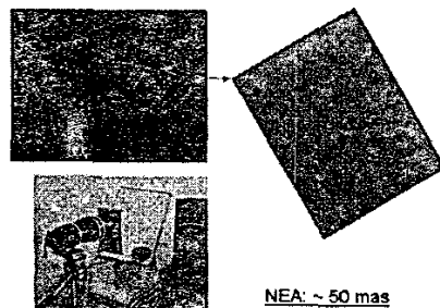
Fig. 1: A 250 mm telescope co-aligned with a CHU. Using the ASCfit algorithm, the attitude of the telescope was measured with a Noise Equivalent Angle (NEA) of 50 mas.
