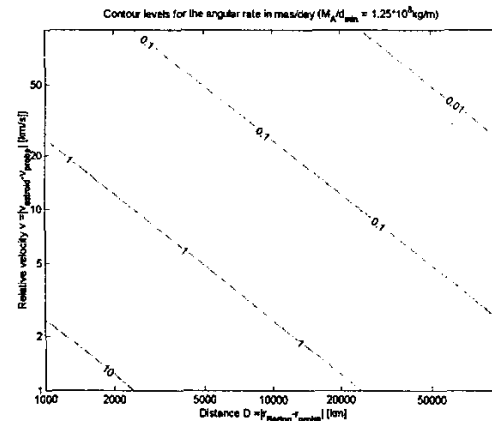
Fig. 5: Estimated post-encounter angular drift-rate.
