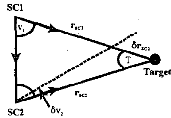
Fig. 8: Accuracy of the range estimate from triangulation.
