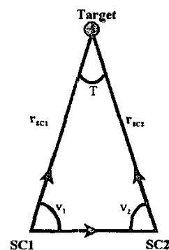
Fig. 7: Basic geometry for the triangulation.
