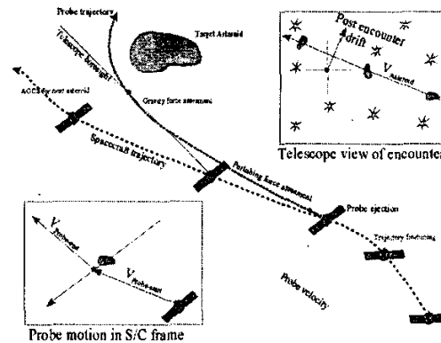
Fig. 4: Principle of mass estimation.
