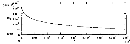
Fig. 3: Theoretical S/N ratio for the detected return pulse versus target distance.
