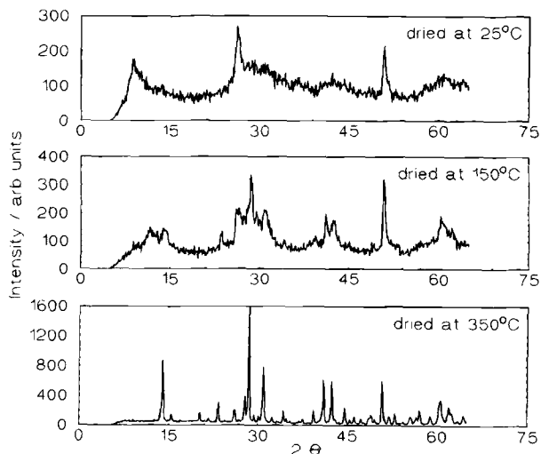
Fig. 3. X-ray diffractograms of lithium trivanadate xerogels made by freeze drying. The as-prepared material is compared with materials heat-treated at 150 and at 350°C.
