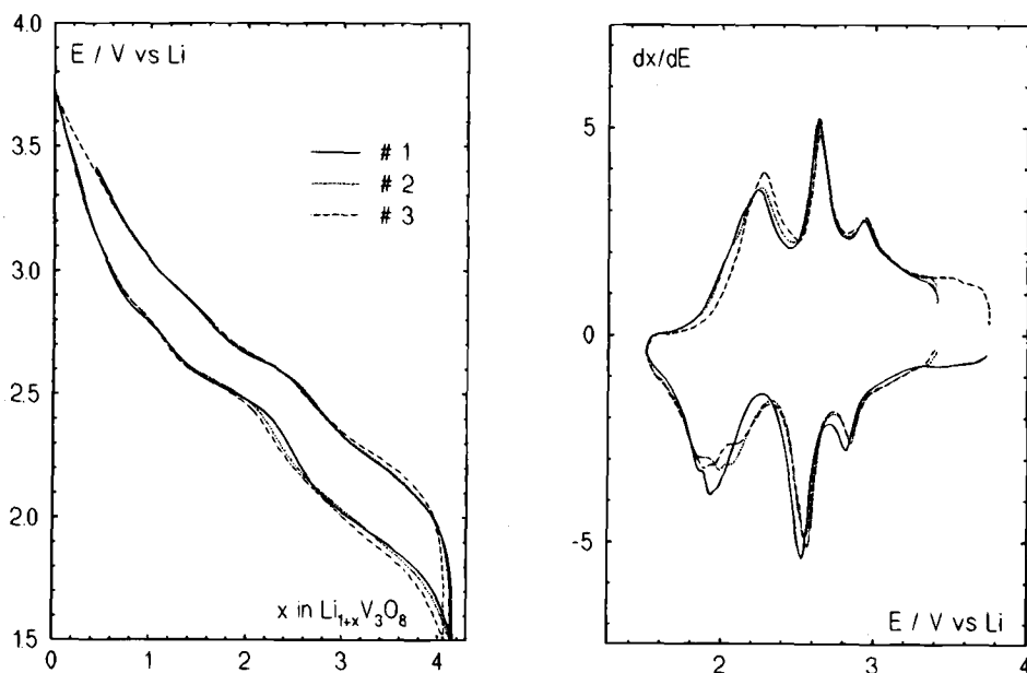
Fig. 7. First three cycles of a cell with lithium trivanadate prepared from spray-dried xerogel, heat-treated at 150°C
