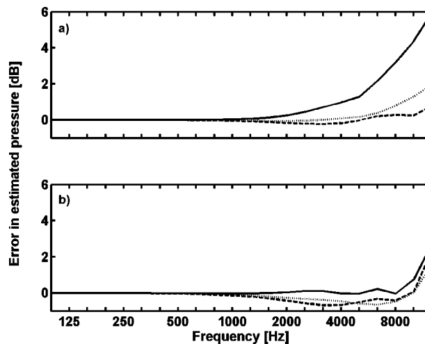
FIG. 8. Error in the estimated sound pressure calculated for (a) a solitary 0.5 in. microphone, and (b) the optimized sound intensity probe, with w = 0.775 .—, 0^\circ ; ---, 90^\circ ; \cdots , diffuse incidence.
