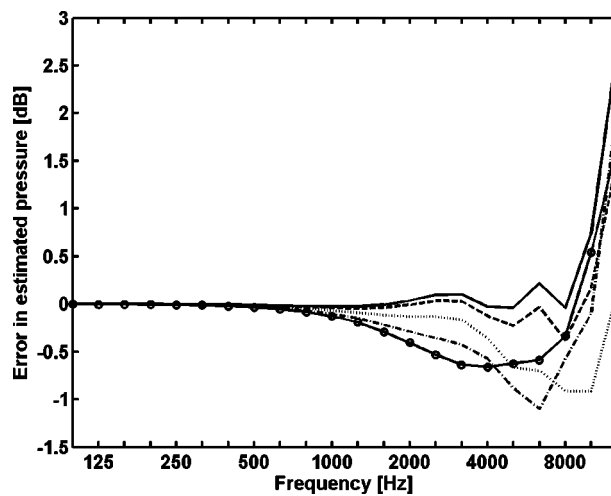
FIG. 7. Error in the estimated sound pressure with w = 0.775 for a plane wave at various angles of incidence:—, 0^\circ ; ---, 20^\circ ; \cdots , 40^\circ ; -·-·-, 60^\circ ; -○-, 80^\circ .
