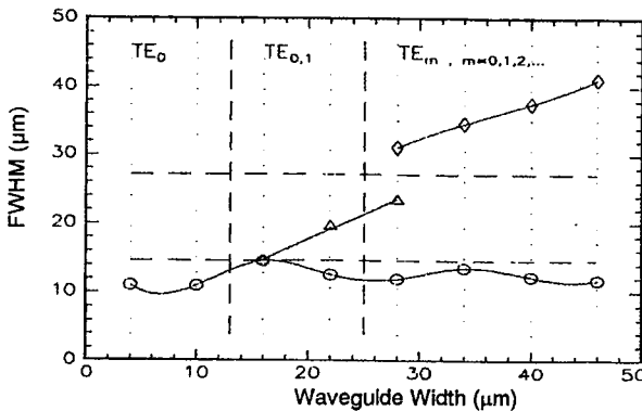
Figure 2. The measured spot size versus width of typical planar silicon optical waveguides made during the course of this work. Note that the first, second, and third order modes are observable in waveguides having widths around 28 \mu\text{m} .
