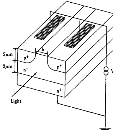
Figure 1. A perspective view of the planar p+n-n+ waveguide structure employed in this work. Note that the optical beam is confined to the region between the two p+ regions on top and the n+ substrate beneath.
