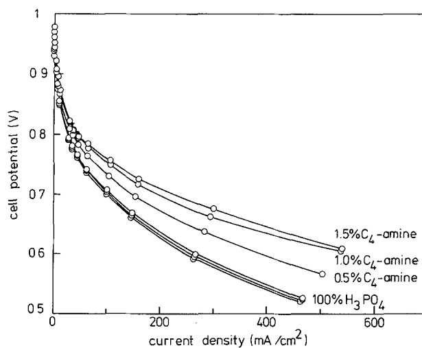
Fig. 9. Polarization curves for electrolyte modified by addition of C 4 -amine (fuel H 2 ; oxidant, O 2 ; electrolyte, 100% H 3 PO 4 ; and temperature, 190°C).
