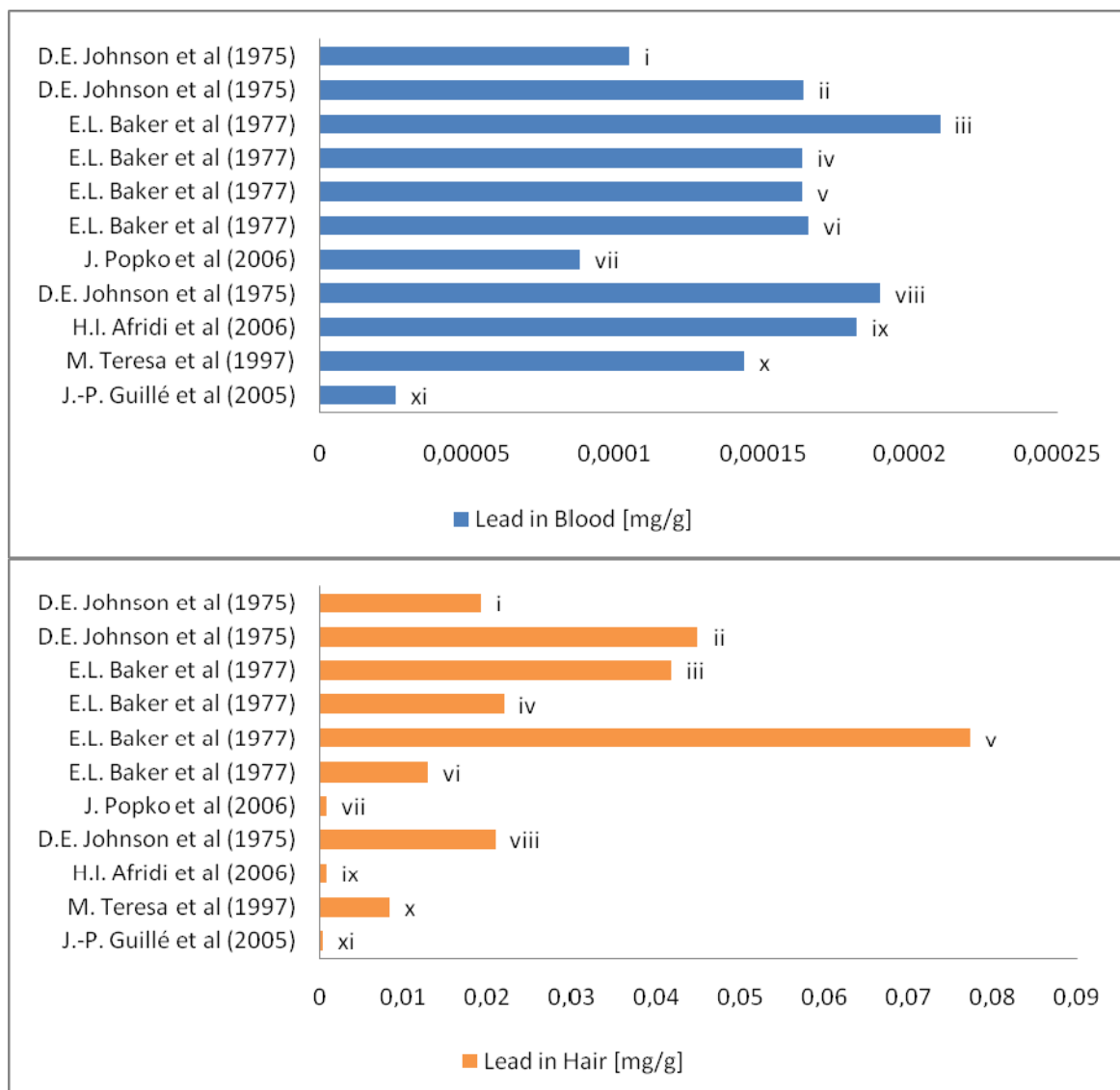
Figure 1. Measurements of stable lead in human blood (blue bars) and human hair (yellow bars) from different studies.
