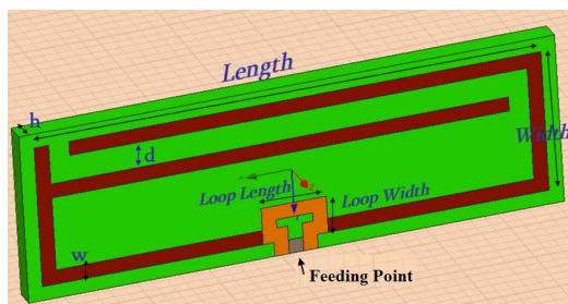
Fig. 1. Geometry of design variables of the self-resonant electrically small loop antenna. (Antenna design 1 for 900 MHz, the dimension is 35mm \times 10mm \times 1.5mm )
