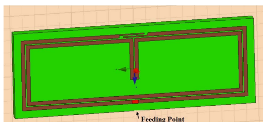
Fig. 2. Geometry of design variables of the self-resonant electrically small split ring antenna. (Antenna design 2 for 900 MHz, the dimension is 36.6mm \times 11.6mm \times 1.5mm )
