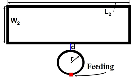
Fig. 7. Circular Small Loop Feeding (Small Loop is Outside).
