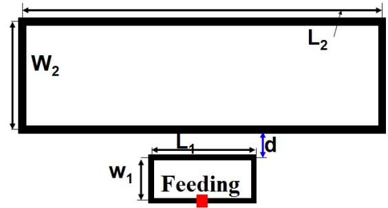
Fig. 4. Rectangular Small Loop Feeding (Small Loop is Outside).
