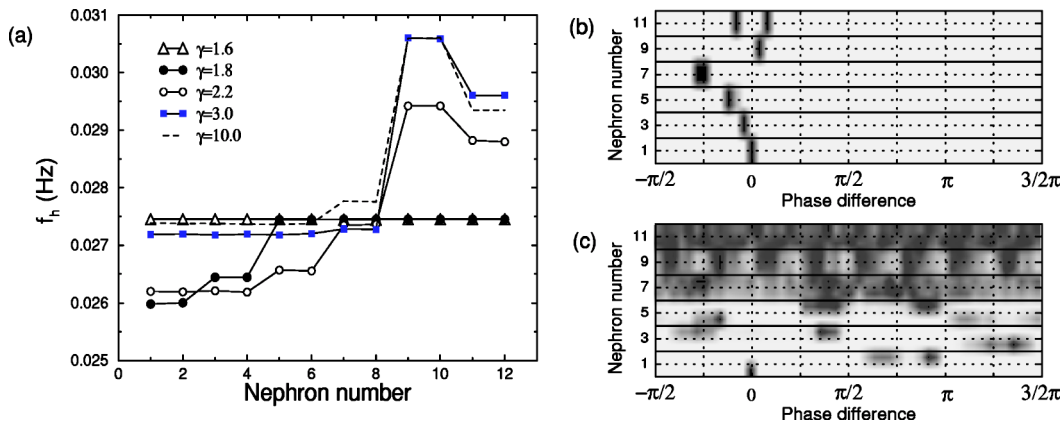
FIG. 10. (a) Slow frequency adjustment for R^b=0.01 \text{ kPa}\cdot\text{s/nl} with varying vascular coupling. Phase entrainment of slow dynamics at (b) \gamma=1.6 \text{ mm}^{-1} ; and (c) \gamma=3.0 \text{ mm}^{-1} . ( R^b=0.01 \text{ kPa}\cdot\text{s/nl} and P_a=13.3 \text{ kPa} ).
