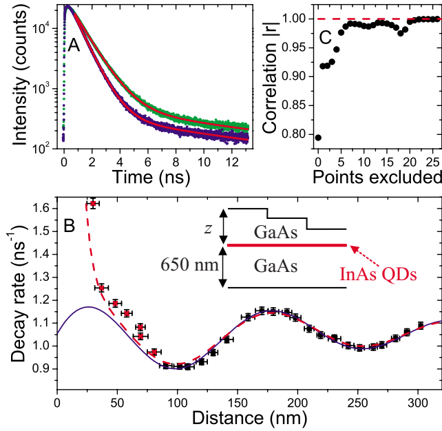
FIG. 1. (Color online) (A) Decay of the spontaneous emission recorded at 1.20 eV for two different distances to the interface of z=109 nm (green/light gray, upper curve) and z=170 nm (blue/dark gray, lower curve). The solid red/gray lines are biexponential fits resulting in \Gamma_f=0.91 ns -1 and \Gamma_s=0.09 ns -1 for z=109 nm and \Gamma_f=1.15 ns -1 and \Gamma_s=0.10 ns -1 for z=170 nm. The goodness-of-fit parameters \chi_r^2 are, respectively, 1.17 and 1.11, close to the ideal value of unity (Ref. 14) verifying the biexponential model. (B) Measured decay rates versus distance z to the GaAs-air interface (squares). Calculated LDOS projected onto a dipole orientation parallel to the interface (solid blue/dark gray line). Calculated LDOS including dissipation at the surface (dashed red/gray line). The inset shows a schematic drawing of the sample. (C) Coefficient of correlation versus the number of data points excluded in the modeling of the data in (B).
