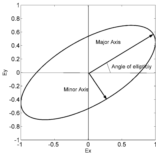
FIG. 2. Projection of the electrical field vector in the x - y plane. The electrical field vector rotates in the mathematically negative direction (from the positive x axis toward the negative y axis) resulting in a right-hand elliptically polarized wave in a right handed coordinate system ( z axis pointing toward the observer).
